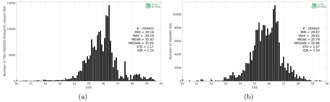
Figure 2: Histograms of SSS from TSG (GOSUD-Research-vessel) (a) and Aquarius SSS L2 OR v5 (NASA-GSFC) (b) considering all match-up pairs per bins of 0.1 over the Mid-Low Latitudes 45N-45S Pi-MEP region and for the full satellite product period.
