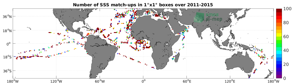
Figure 4: Number of SSS match-ups between TSG (GOSUD-Research-vessel) SSS and the Aquarius SSS L2 OR v5 (NASA-GSFC) SSS product for the Mid-Low Latitudes 45N-45S Pi-MEP region over 1^\circ \times 1^\circ boxes and for the full satellite product period.
