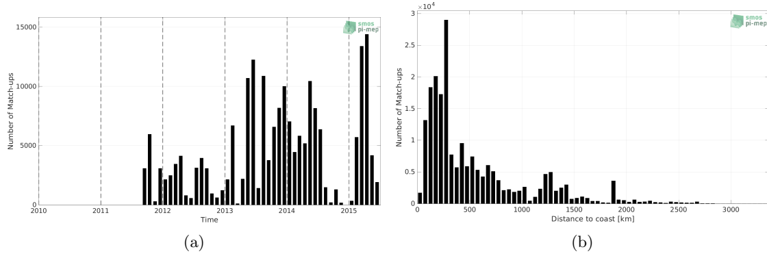
Figure 1: Number of match-ups between TSG (GOSUD-Research-vessel) and Aquarius SSS L2 OR v5 (NASA-GSFC) SSS as a function of time (a) and as function of the distance to coast (b) over the Mid-Low Latitudes 45N-45S Pi-MEP region and for the full satellite product period.
