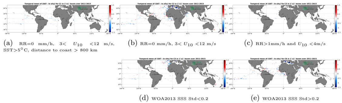
Figure 12: Temporal mean gridded over spatial boxes of size 1^\circ \times 1^\circ of \Delta\text{SSS} (Aquarius SSS L2 OR v5 (NASA-GSFC) - TSG (GOSUD-Research-vessel)) for 5 different subdatasets corresponding to: RR=0 mm/h, 3 < U_{10} < 12 m/s, SST > 5°C, distance to coast > 800 km (a), RR=0 mm/h, 3 < U_{10} < 12 m/s (b), RR > 1mm/h and U_{10} < 4 m/s (c), WOA2013 SSS Std < 0.2 (d), WOA2013 SSS Std > 0.2 (e).
