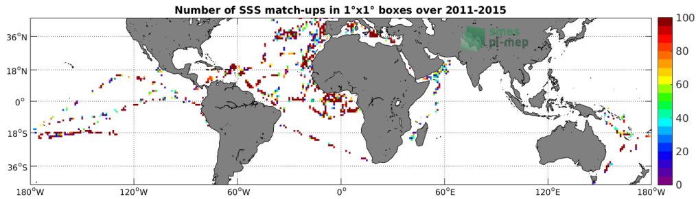
Figure 4: Number of SSS match-ups between TSG-GOSUD-Research-vessel SSS and the Aquarius-L2-OR-V5 SSS product for the Mid-Low Latitudes 45N-45S Pi-MEP region over 1^\circ \times 1^\circ boxes and for the full satellite product period.
