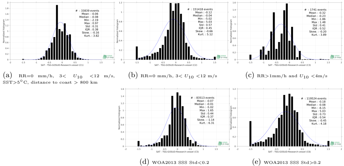
Figure 13: Normalized histogram of \Delta SSS (Aquarius-L2-OR-V5 - TSG-GOSUD-Research-vessel) for 5 different subdatasets corresponding to: RR=0 mm/h, 3 < U_{10} < 12 m/s, SST >5^\circ\text{C} , distance to coast > 800 km (a), RR=0 mm/h, 3 < U_{10} < 12 m/s (b), RR >1 mm/h and U_{10} < 4 m/s (c), WOA2013 SSS Std <0.2 (d), WOA2013 SSS Std >0.2 (e).
