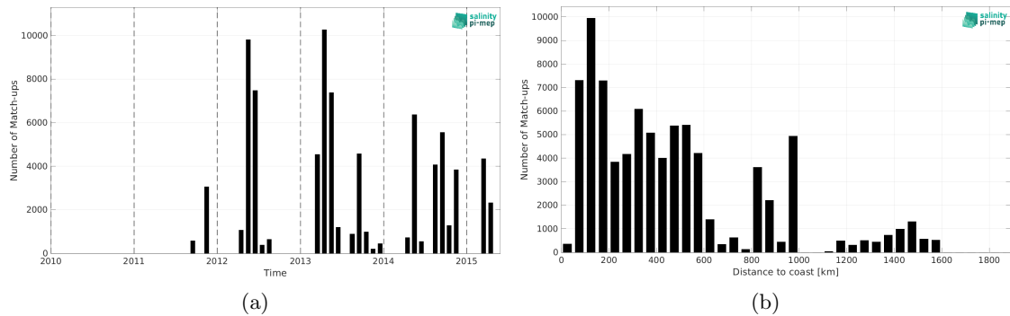
Figure 2: Number of match-ups between TSG (CSIC-UTM) and Aquarius SSS L2 OR v5 (NASA-GSFC) SSS as a function of time (a) and as function of the distance to coast (b) over the Mid-Low Latitudes 45N-45S Pi-MEP region and for the full satellite product period.
