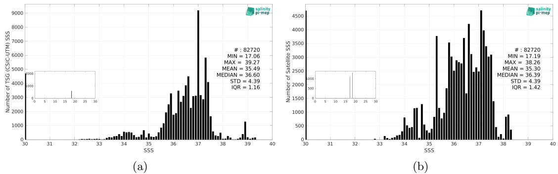
Figure 3: Histograms of SSS from TSG (CSIC-UTM) (a) and Aquarius SSS L2 OR v5 (NASA-GSFC) (b) considering all match-up pairs per bins of 0.1 over the Mid-Low Latitudes 45N-45S Pi-MEP region and for the full satellite product period.
