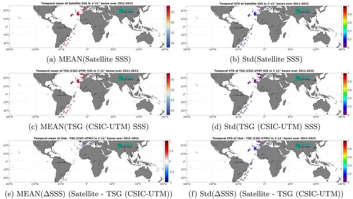
Figure 7: Temporal mean (left) and Std (right) of SSS from Aquarius SSS L2 OR v5 (NASA-GSFC) (top), TSG (CSIC-UTM) (middle), and of \Delta SSS (Satellite - TSG (CSIC-UTM)). Only match-up pairs are used to generate these maps.
