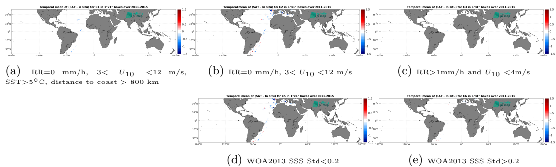
Figure 14: Temporal mean gridded over spatial boxes of size 1^\circ \times 1^\circ of \Delta\text{SSS} (Aquarius SSS L2 OR v5 (NASA-GSFC) - TSG (CSIC-UTM)) for 5 different subdatasets corresponding to: RR=0 mm/h, 3 < U_{10} < 12 m/s, SST > 5°C, distance to coast > 800 km (a), RR=0 mm/h, 3 < U_{10} < 12 m/s (b), RR > 1mm/h and U_{10} < 4 m/s (c), WOA2013 SSS Std < 0.2 (d), WOA2013 SSS Std > 0.2 (e).
