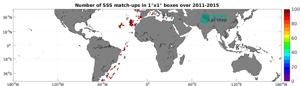
Figure 5: Number of SSS match-ups between TSG (CSIC-UTM) SSS and the Aquarius SSS L2 OR v5 (NASA-GSFC) SSS product for the Mid-Low Latitudes 45N-45S Pi-MEP region over 1^\circ \times 1^\circ boxes and for the full satellite product period.
