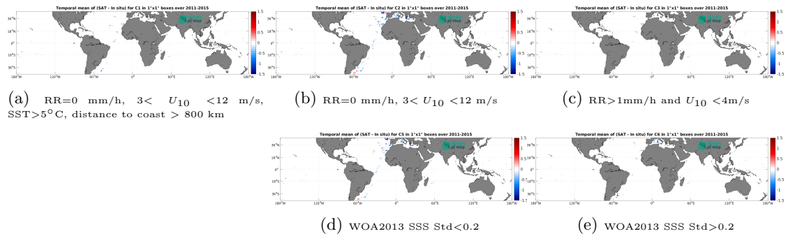
Figure 12: Temporal mean gridded over spatial boxes of size 1^\circ \times 1^\circ of \Delta\text{SSS} (Aquarius SSS L2 OR v5 (NASA-GSFC) - TSG (CSIC-UTM)) for 5 different subdatasets corresponding to: RR=0 mm/h, 3 < U_{10} < 12 m/s, SST > 5^\circ\text{C} , distance to coast > 800 km (a), RR=0 mm/h, 3 < U_{10} < 12 m/s (b), RR > 1\text{mm/h} and U_{10} < 4\text{m/s} (c), WOA2013 SSS Std < 0.2 (d), WOA2013 SSS Std > 0.2 (e).
