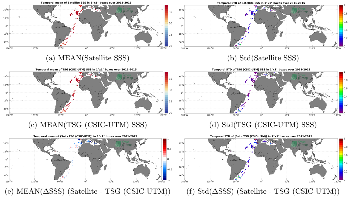
Figure 6: Temporal mean (left) and Std (right) of SSS from Aquarius SSS L2 OR v5 (NASA-GSFC) (top), TSG (CSIC-UTM) (middle), and of \Delta SSS (Satellite - TSG (CSIC-UTM)). Only match-up pairs are used to generate these maps.
