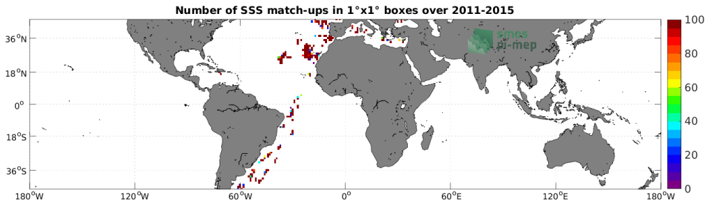
Figure 4: Number of SSS match-ups between TSG (CSIC-UTM) SSS and the Aquarius SSS L2 OR v5 (NASA-GSFC) SSS product for the Mid-Low Latitudes 45N-45S Pi-MEP region over 1^\circ \times 1^\circ boxes and for the full satellite product period.
