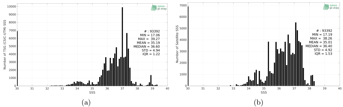
Figure 2: Histograms of SSS from TSG (CSIC-UTM) (a) and Aquarius SSS L2 OR v5 (NASA-GSFC) (b) considering all match-up pairs per bins of 0.1 over the Mid-Low Latitudes 45N-45S Pi-MEP region and for the full satellite product period.
