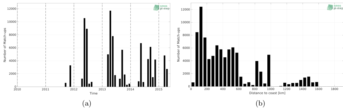
Figure 1: Number of match-ups between TSG (CSIC-UTM) and Aquarius SSS L2 OR v5 (NASA-GSFC) SSS as a function of time (a) and as function of the distance to coast (b) over the Mid-Low Latitudes 45N-45S Pi-MEP region and for the full satellite product period.
