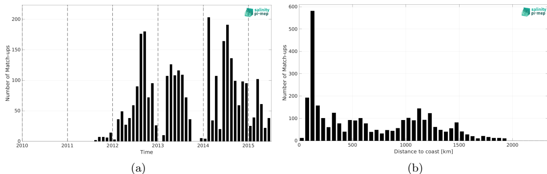
Figure 2: Number of match-ups between Marine mammals and Aquarius SSS L2 OR v5 (NASA-GSFC) SSS as a function of time (a) and as function of the distance to coast (b) over the Mid-Low Latitudes 45N-45S Pi-MEP region and for the full satellite product period.
