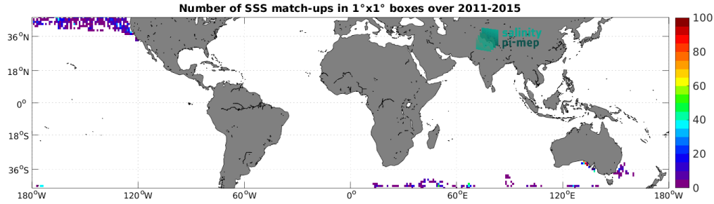
Figure 5: Number of SSS match-ups between Marine mammals SSS and the Aquarius SSS L2 OR v5 (NASA-GSFC) SSS product for the Mid-Low Latitudes 45N-45S Pi-MEP region over 1^\circ \times 1^\circ boxes and for the full satellite product period.
