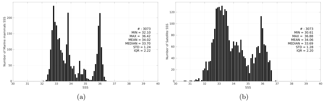
Figure 3: Histograms of SSS from Marine mammals (a) and Aquarius SSS L2 OR v5 (NASA-GSFC) (b) considering all match-up pairs per bins of 0.1 over the Mid-Low Latitudes 45N-45S Pi-MEP region and for the full satellite product period.
