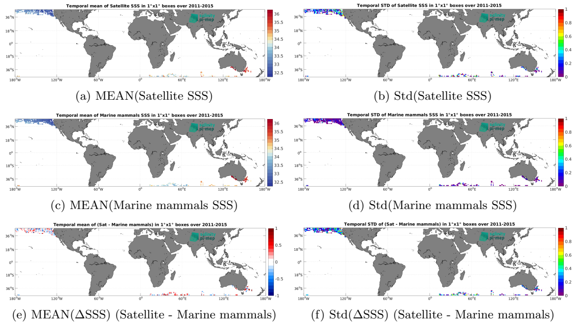
Figure 7: Temporal mean (left) and Std (right) of SSS from Aquarius SSS L2 OR v5 (NASA-GSFC) (top), Marine mammals (middle), and of \Delta SSS (Satellite - Marine mammals). Only match-up pairs are used to generate these maps.
