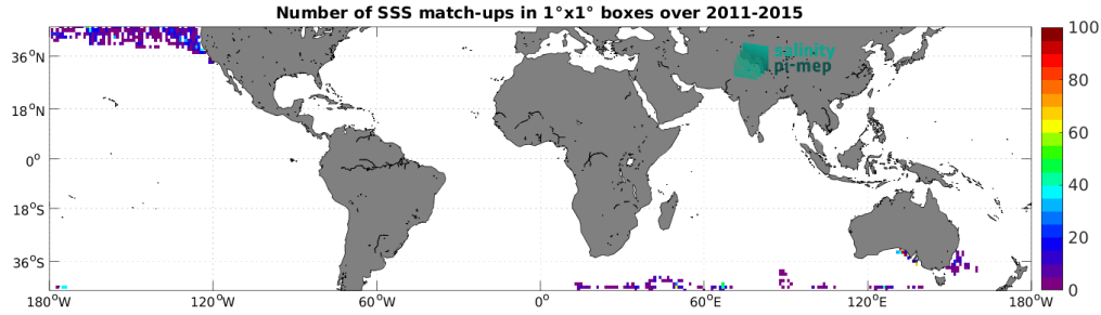
Figure 4: Number of SSS match-ups between Marine mammals SSS and the Aquarius SSS L2 OR v5 (NASA-GSFC) SSS product for the Mid-Low Latitudes 45N-45S Pi-MEP region over 1^\circ \times 1^\circ boxes and for the full satellite product period.
