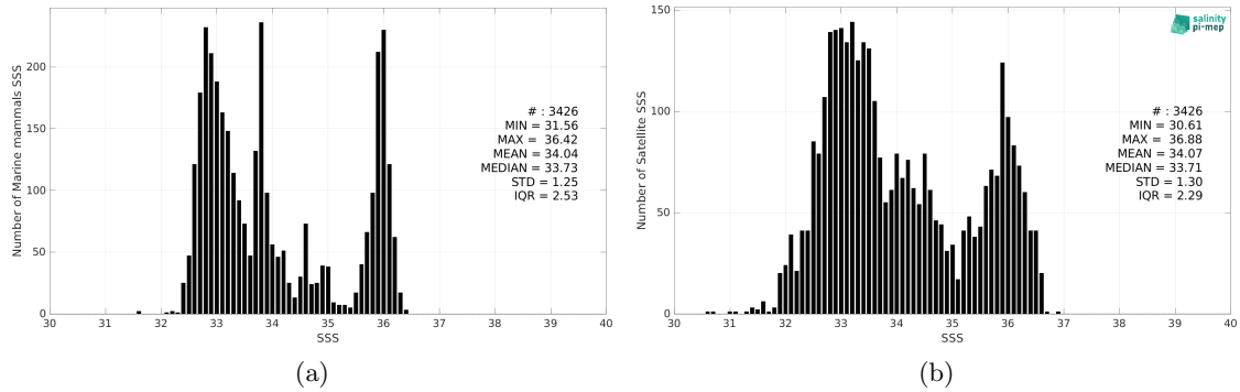
Figure 2: Histograms of SSS from Marine mammals (a) and Aquarius SSS L2 OR v5 (NASA-GSFC) (b) considering all match-up pairs per bins of 0.1 over the Mid-Low Latitudes 45N-45S Pi-MEP region and for the full satellite product period.
