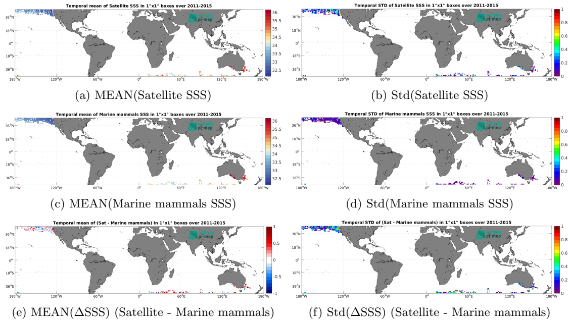
Figure 6: Temporal mean (left) and Std (right) of SSS from Aquarius SSS L2 OR v5 (NASA-GSFC) (top), Marine mammals (middle), and of \Delta SSS (Satellite - Marine mammals). Only match-up pairs are used to generate these maps.
