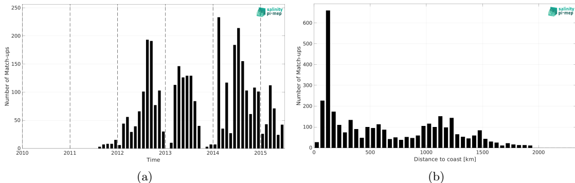
Figure 1: Number of match-ups between Marine mammals and Aquarius SSS L2 OR v5 (NASA-GSFC) SSS as a function of time (a) and as function of the distance to coast (b) over the Mid-Low Latitudes 45N-45S Pi-MEP region and for the full satellite product period.
