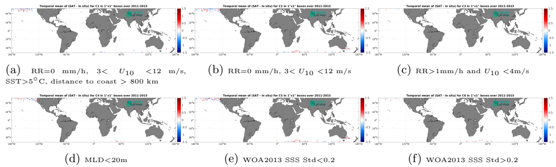
Figure 12: Temporal mean gridded over spatial boxes of size 1^\circ \times 1^\circ of \Delta SSS (Aquarius SSS L2 OR v5 (NASA-GSFC) - Marine mammals) for 6 different subdatasets corresponding to:RR=0 mm/h, 3 < U_{10} < 12 m/s, SST >5^\circ C, distance to coast > 800 km (a), RR=0 mm/h, 3 < U_{10} < 12 m/s (b), RR >1 mm/h and U_{10} < 4 m/s (c),MLD <20 m (d),WOA2013 SSS Std <0.2 (e),WOA2013 SSS Std >0.2 (f).
