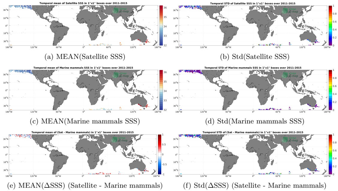
Figure 6: Temporal mean (left) and Std (right) of SSS from Aquarius SSS L2 OR v5 (NASA-GSFC) (top), Marine mammals (middle), and of \Delta SSS (Satellite - Marine mammals). Only match-up pairs are used to generate these maps.
