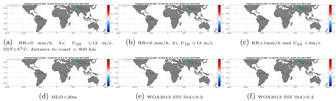
Figure 12: Temporal mean gridded over spatial boxes of size 1^\circ \times 1^\circ of \Delta SSS (Aquarius-L2-OR-V5 - Sea mammals) for 6 different subdatasets corresponding to:RR=0 mm/h, 3 < U_{10} < 12 m/s, SST >5^\circ C, distance to coast > 800 km (a), RR=0 mm/h, 3 < U_{10} < 12 m/s (b), RR >1 mm/h and U_{10} < 4 m/s (c),MLD <20 m (d),WOA2013 SSS Std <0.2 (e),WOA2013 SSS Std >0.2 (f).
