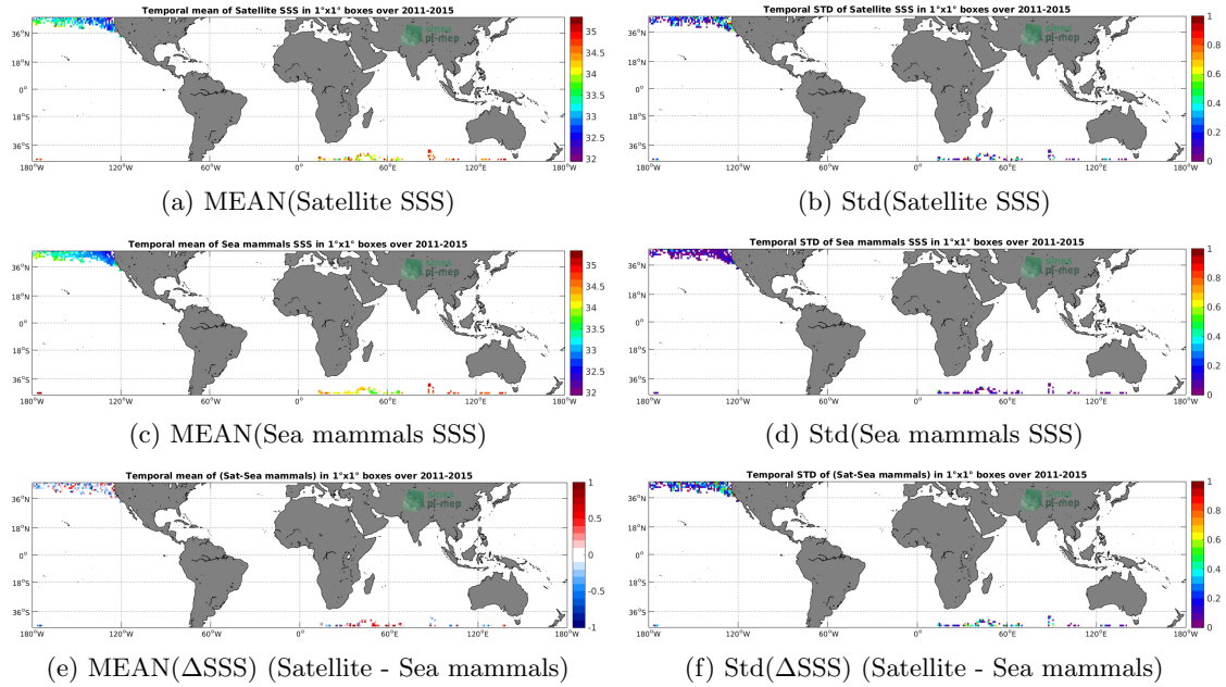
Figure 6: Temporal mean (left) and Std (right) of SSS from Aquarius-L2-OR-V5 (top), Sea mammals (middle), and of \Delta SSS (Satellite - Sea mammals). Only match-up pairs are used to generate these maps.
