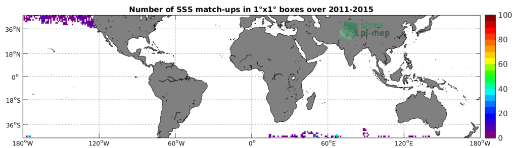
Figure 4: Number of SSS match-ups between Sea mammals SSS and the Aquarius-L2-OR-V5 SSS product for the Mid-Low Latitudes 45N-45S Pi-MEP region over 1°x1° boxes and for the full satellite product period.
