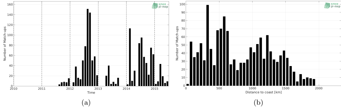
Figure 1: Number of match-ups between Sea mammals and Aquarius-L2-OR-V5 SSS as a function of time (a) and as function of the distance to coast (b) over the Mid-Low Latitudes 45N-45S Pi-MEP region and for the full satellite product period.
