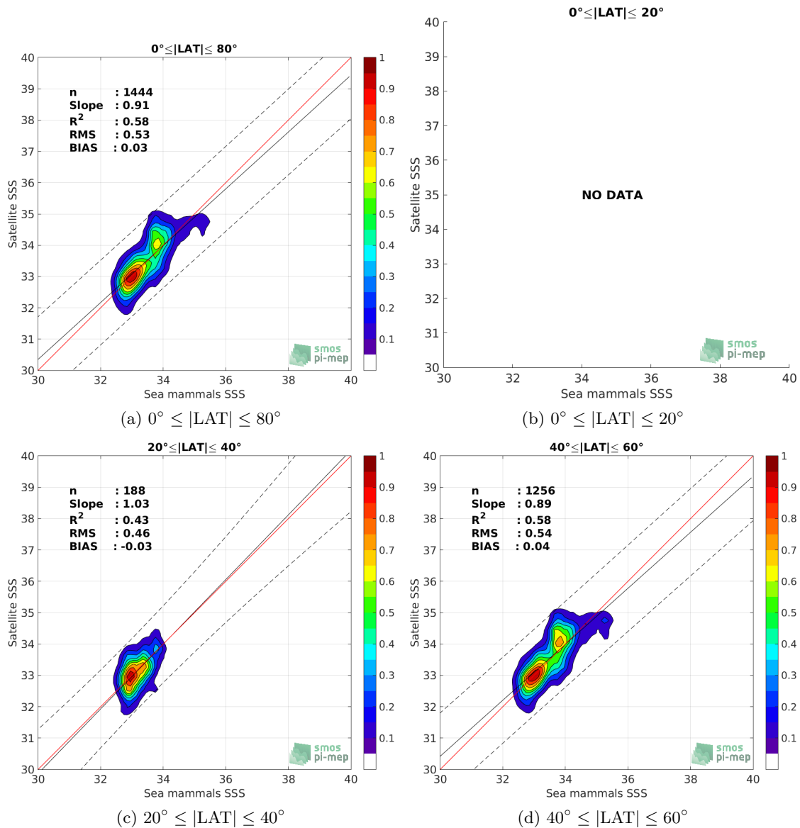
Figure 9: Contour maps of the concentration of Aquarius-L2-OR-V5 SSS (y-axis) versus Sea mammals SSS (x-axis) at match-up pairs for different latitude bands. For each plot, the red line shows x=y . The black thin and dashed lines indicate a linear fit through the data cloud and the \pm 95\% confidence levels, respectively. The number match-up pairs n , the slope and R^2 coefficient of the linear fit, the root mean square (RMS) and the mean bias between satellite and in situ data are indicated for each latitude band in each plots.
