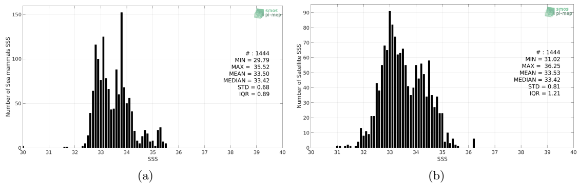
Figure 2: Histograms of SSS from Sea mammals (a) and Aquarius-L2-OR-V5 (b) considering all match-up pairs per bins of 0.1 over the Mid-Low Latitudes 45N-45S Pi-MEP region and for the full satellite product period.
