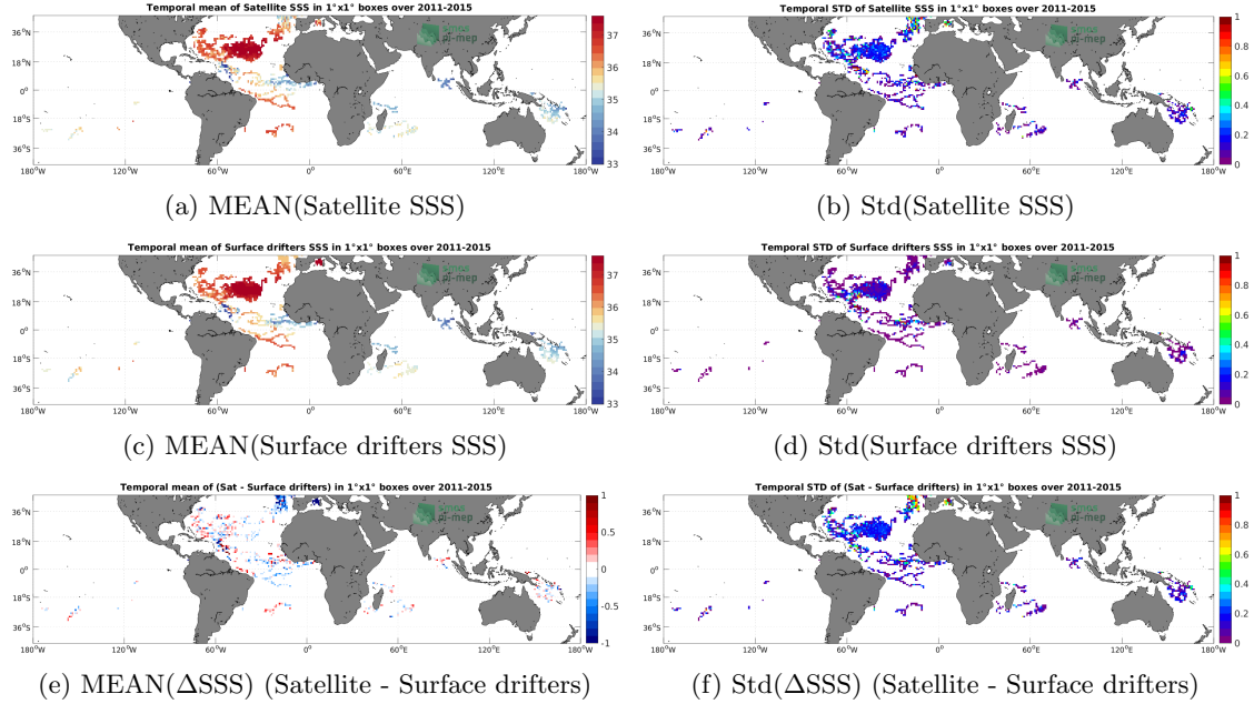
Figure 5: Temporal mean (left) and Std (right) of SSS from Aquarius SSS L2 OR v5 (NASA-GSFC) (top), Surface drifters (middle), and of \Delta SSS (Satellite - Surface drifters). Only match-up pairs are used to generate these maps.
