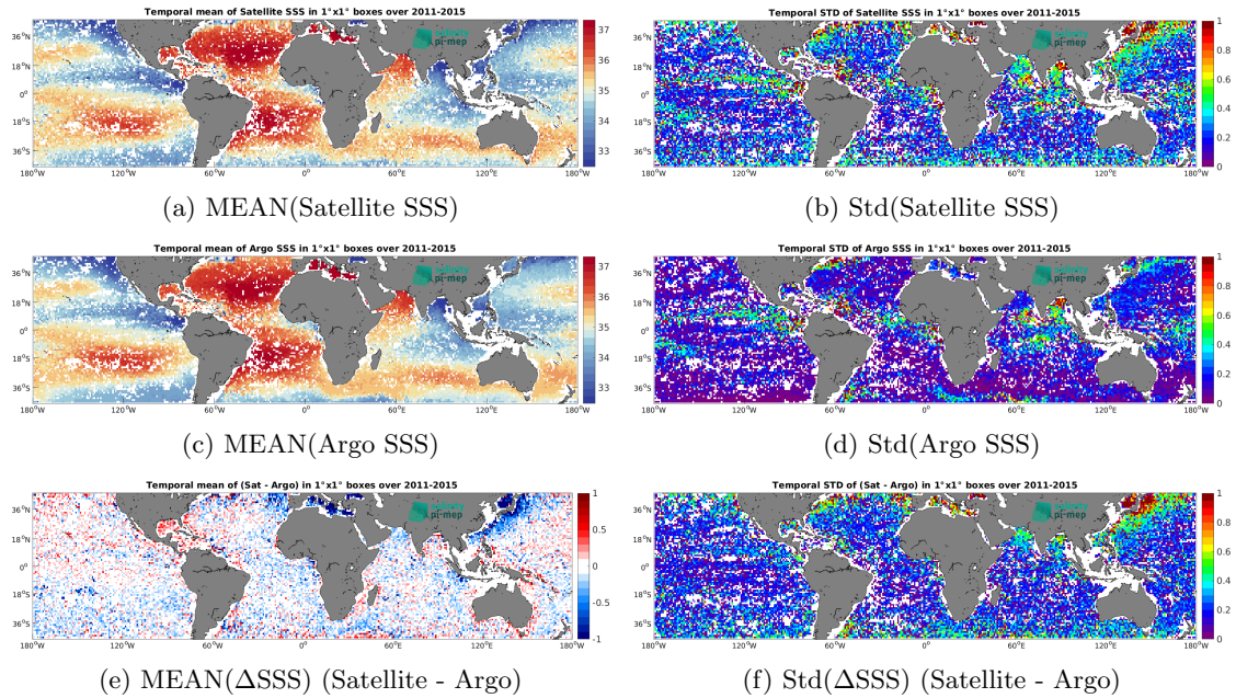
Figure 7: Temporal mean (left) and Std (right) of SSS from Aquarius SSS L2 OR v5 (NASA-GSFC) (top), Argo (middle), and of \Delta SSS (Satellite - Argo). Only match-up pairs are used to generate these maps.
