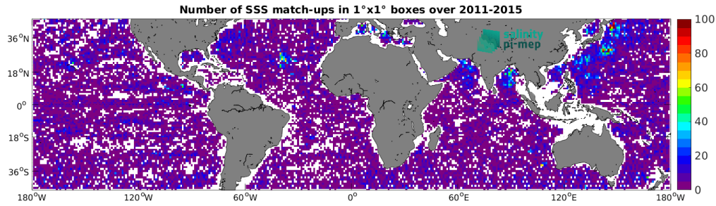
Figure 5: Number of SSS match-ups between Argo SSS and the Aquarius SSS L2 OR v5 (NASA-GSFC) SSS product for the Mid-Low Latitudes 45N-45S Pi-MEP region over 1^\circ \times 1^\circ boxes and for the full satellite product period.
