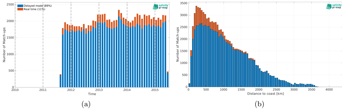
Figure 2: Number of match-ups between Argo and Aquarius SSS L2 OR v5 (NASA-GSFC) SSS as a function of time (a) and as function of the distance to coast (b) over the Mid-Low Latitudes 45N-45S Pi-MEP region and for the full satellite product period.
