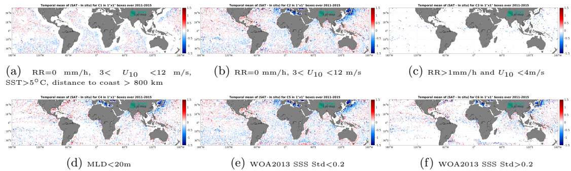
Figure 14: Temporal mean gridded over spatial boxes of size 1^\circ \times 1^\circ of \Delta SSS (Aquarius SSS L2 OR v5 (NASA-GSFC) - Argo) for 6 different subdatasets corresponding to:RR=0 mm/h, 3 < U_{10} < 12 m/s, SST >5^\circ C, distance to coast > 800 km (a), RR=0 mm/h, 3 < U_{10} < 12 m/s (b), RR >1 mm/h and U_{10} < 4 m/s (c),MLD <20 m (d),WOA2013 SSS Std <0.2 (e),WOA2013 SSS Std >0.2 (f).
