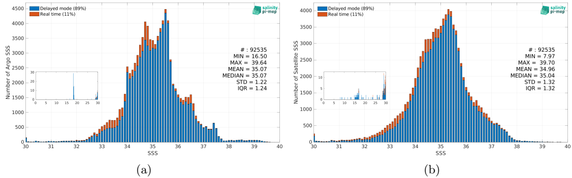
Figure 3: Histograms of SSS from Argo (a) and Aquarius SSS L2 OR v5 (NASA-GSFC) (b) considering all match-up pairs per bins of 0.1 over the Mid-Low Latitudes 45N-45S Pi-MEP region and for the full satellite product period.
