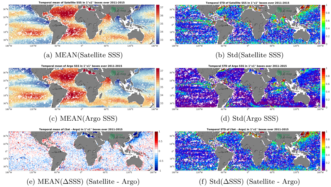
Figure 6: Temporal mean (left) and Std (right) of SSS from Aquarius SSS L2 OR v5 (NASA-GSFC) (top), Argo (middle), and of \Delta SSS (Satellite - Argo). Only match-up pairs are used to generate these maps.
