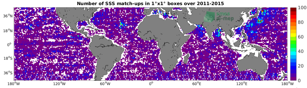
Figure 4: Number of SSS match-ups between Argo SSS and the Aquarius SSS L2 OR v5 (NASA-GSFC) SSS product for the Mid-Low Latitudes 45N-45S Pi-MEP region over 1^\circ \times 1^\circ boxes and for the full satellite product period.
