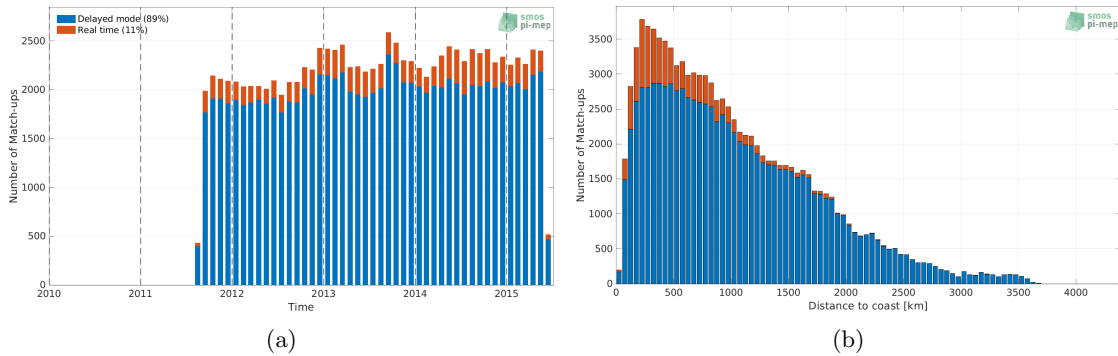
Figure 1: Number of match-ups between Argo and Aquarius SSS L2 OR v5 (NASA-GSFC) SSS as a function of time (a) and as function of the distance to coast (b) over the Mid-Low Latitudes 45N-45S Pi-MEP region and for the full satellite product period.
