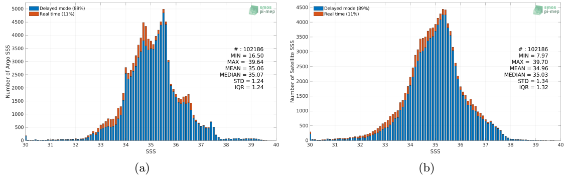
Figure 2: Histograms of SSS from Argo (a) and Aquarius SSS L2 OR v5 (NASA-GSFC) (b) considering all match-up pairs per bins of 0.1 over the Mid-Low Latitudes 45N-45S Pi-MEP region and for the full satellite product period.
