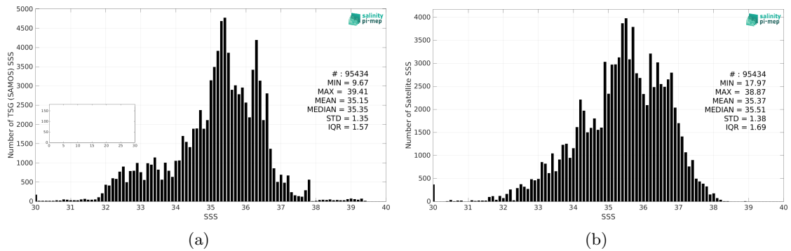
Figure 2: Histograms of SSS from TSG (SAMOS) (a) and Aquarius SSS L2 CAP v5 (JPL) (b) considering all match-up pairs per bins of 0.1 over the Mid-Low Latitudes 45N-45S Pi-MEP region and for the full satellite product period.
