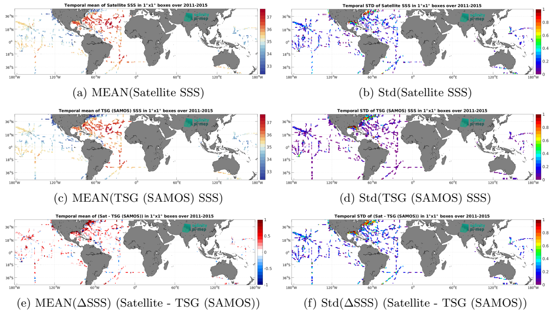
Figure 6: Temporal mean (left) and Std (right) of SSS from Aquarius SSS L2 CAP v5 (JPL) (top), TSG (SAMOS) (middle), and of \Delta SSS (Satellite - TSG (SAMOS)). Only match-up pairs are used to generate these maps.
