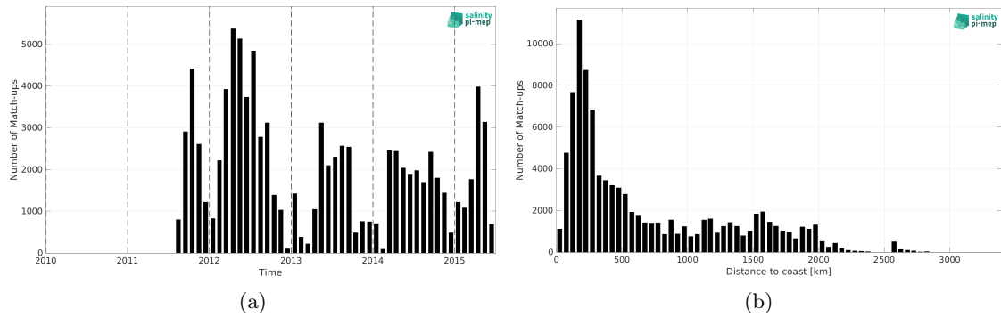
Figure 1: Number of match-ups between TSG (SAMOS) and Aquarius SSS L2 CAP v5 (JPL) SSS as a function of time (a) and as function of the distance to coast (b) over the Mid-Low Latitudes 45N-45S Pi-MEP region and for the full satellite product period.
