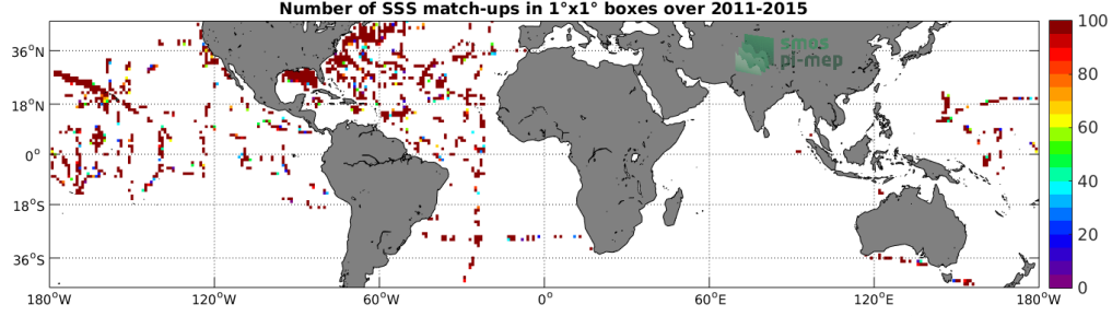
Figure 4: Number of SSS match-ups between TSG-SAMOS SSS and the Aquarius-L2-JPL-V5 SSS product for the Mid-Low Latitudes 45N-45S Pi-MEP region over 1°x1° boxes and for the full satellite product period.
