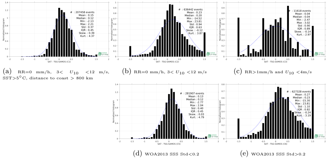
Figure 13: Normalized histogram of \Delta SSS (Aquarius-L2-JPL-V5 - TSG-SAMOS) for 5 different subdatasets corresponding to: RR=0 mm/h, 3 < U_{10} < 12 m/s, SST >5^\circ\text{C} , distance to coast > 800 km (a), RR=0 mm/h, 3 < U_{10} < 12 m/s (b), RR >1 mm/h and U_{10} < 4 m/s (c), WOA2013 SSS Std <0.2 (d), WOA2013 SSS Std >0.2 (e).
