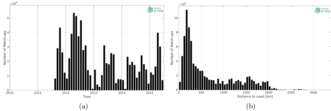
Figure 1: Number of match-ups between TSG-SAMOS and Aquarius-L2-JPL-V5 SSS as a function of time (a) and as function of the distance to coast (b) over the Mid-Low Latitudes 45N-45S Pi-MEP region and for the full satellite product period.
