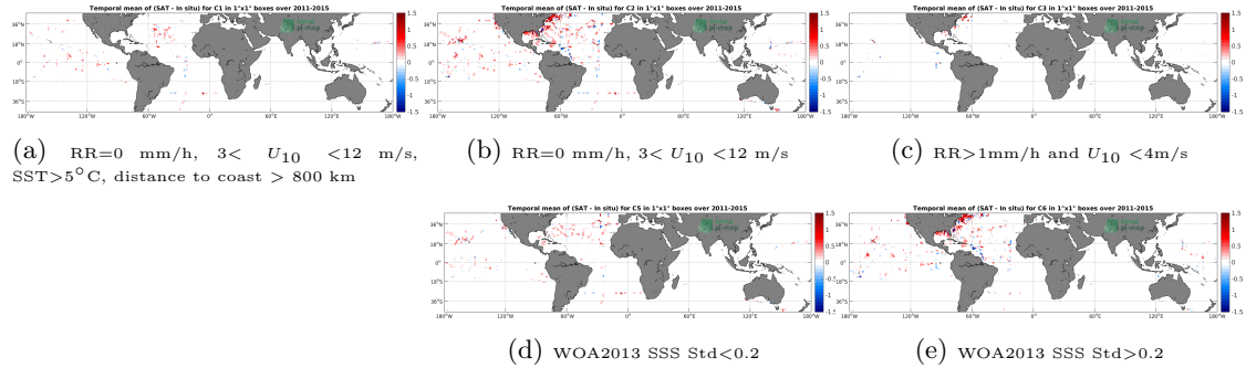
Figure 12: Temporal mean gridded over spatial boxes of size 1^\circ \times 1^\circ of \Delta SSS (Aquarius-L2-JPL-V5 - TSG-SAMOS) for 5 different subdatasets corresponding to: RR=0 mm/h, 3 < U_{10} < 12 m/s, SST >5^\circ C, distance to coast > 800 km (a), RR=0 mm/h, 3 < U_{10} < 12 m/s (b), RR >1 mm/h and U_{10} < 4 m/s (c), WOA2013 SSS Std <0.2 (d), WOA2013 SSS Std >0.2 (e).
