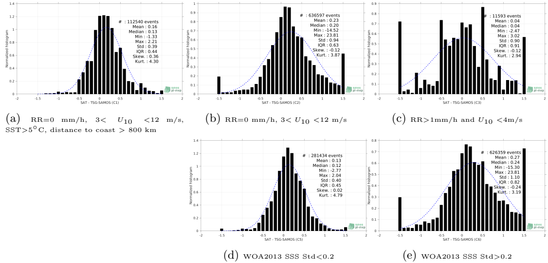
Figure 13: Normalized histogram of \Delta SSS (Aquarius-L2-JPL-V5 - TSG-SAMOS) for 5 different subdatasets corresponding to: RR=0 mm/h, 3 < U_{10} < 12 m/s, SST >5^\circ C, distance to coast > 800 km (a), RR=0 mm/h, 3 < U_{10} < 12 m/s (b), RR >1 mm/h and U_{10} < 4 m/s (c), WOA2013 SSS Std <0.2 (d), WOA2013 SSS Std >0.2 (e).
