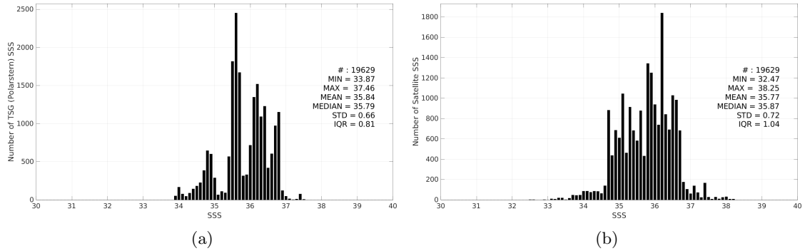
Figure 3: Histograms of SSS from TSG (Polarstern) (a) and Aquarius SSS L2 CAP v5 (JPL) (b) considering all match-up pairs per bins of 0.1 over the Mid-Low Latitudes 45N-45S Pi-MEP region and for the full satellite product period.
