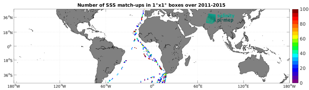
Figure 5: Number of SSS match-ups between TSG (Polarstern) SSS and the Aquarius SSS L2 CAP v5 (JPL) SSS product for the Mid-Low Latitudes 45N-45S Pi-MEP region over 1^\circ \times 1^\circ boxes and for the full satellite product period.
