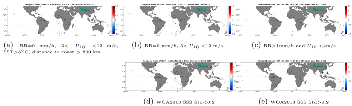
Figure 14: Temporal mean gridded over spatial boxes of size 1^\circ \times 1^\circ of \Delta SSS (Aquarius SSS L2 CAP v5 (JPL) - TSG (Polarstern)) for 5 different subdatasets corresponding to: RR=0 mm/h, 3 < U_{10} < 12 m/s, SST > 5°C, distance to coast > 800 km (a), RR=0 mm/h, 3 < U_{10} < 12 m/s (b), RR > 1mm/h and U_{10} < 4 m/s (c), WOA2013 SSS Std < 0.2 (d), WOA2013 SSS Std > 0.2 (e).
