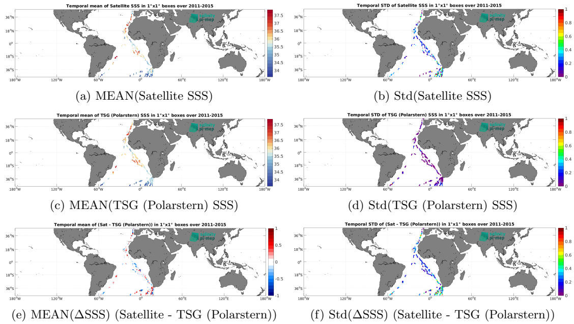
Figure 7: Temporal mean (left) and Std (right) of SSS from Aquarius SSS L2 CAP v5 (JPL) (top), TSG (Polarstern) (middle), and of \Delta SSS (Satellite - TSG (Polarstern)). Only match-up pairs are used to generate these maps.
