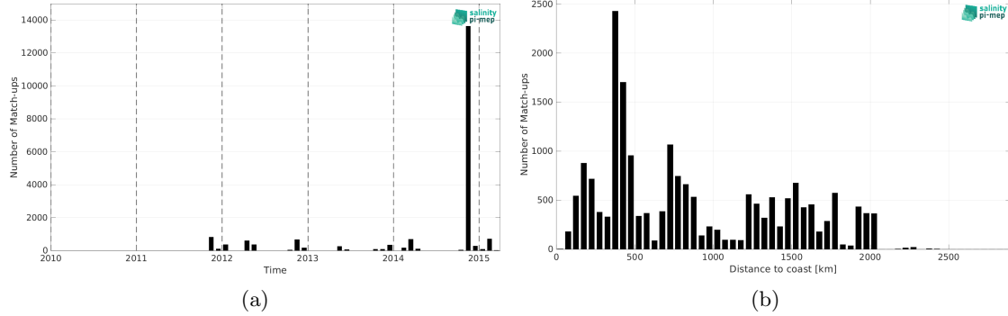
Figure 2: Number of match-ups between TSG (Polarstern) and Aquarius SSS L2 CAP v5 (JPL) SSS as a function of time (a) and as function of the distance to coast (b) over the Mid-Low Latitudes 45N-45S Pi-MEP region and for the full satellite product period.
