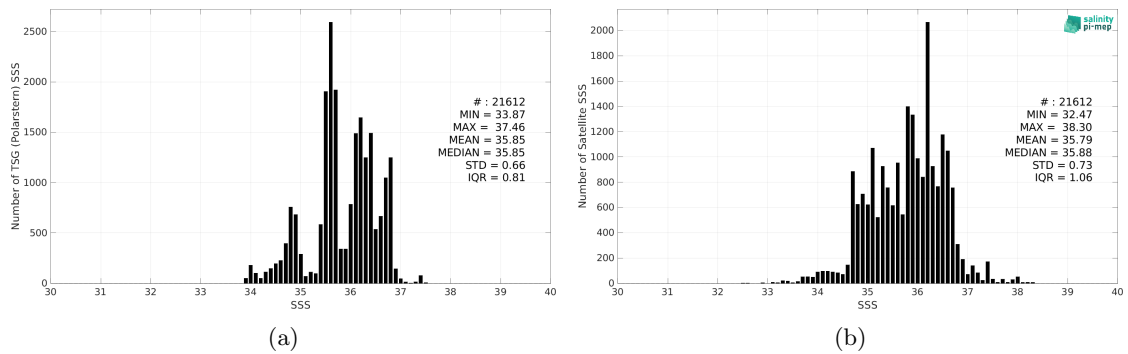
Figure 2: Histograms of SSS from TSG (Polarstern) (a) and Aquarius SSS L2 CAP v5 (JPL) (b) considering all match-up pairs per bins of 0.1 over the Mid-Low Latitudes 45N-45S Pi-MEP region and for the full satellite product period.
