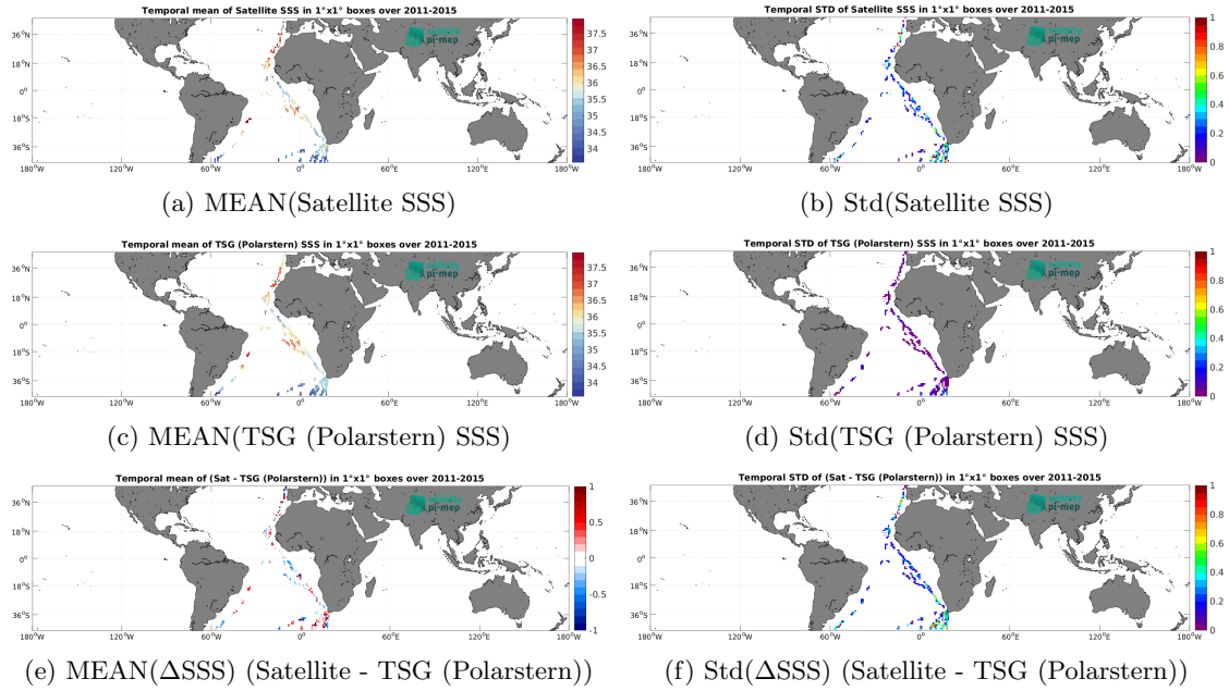
Figure 6: Temporal mean (left) and Std (right) of SSS from Aquarius SSS L2 CAP v5 (JPL) (top), TSG (Polarstern) (middle), and of \Delta SSS (Satellite - TSG (Polarstern)). Only match-up pairs are used to generate these maps.
