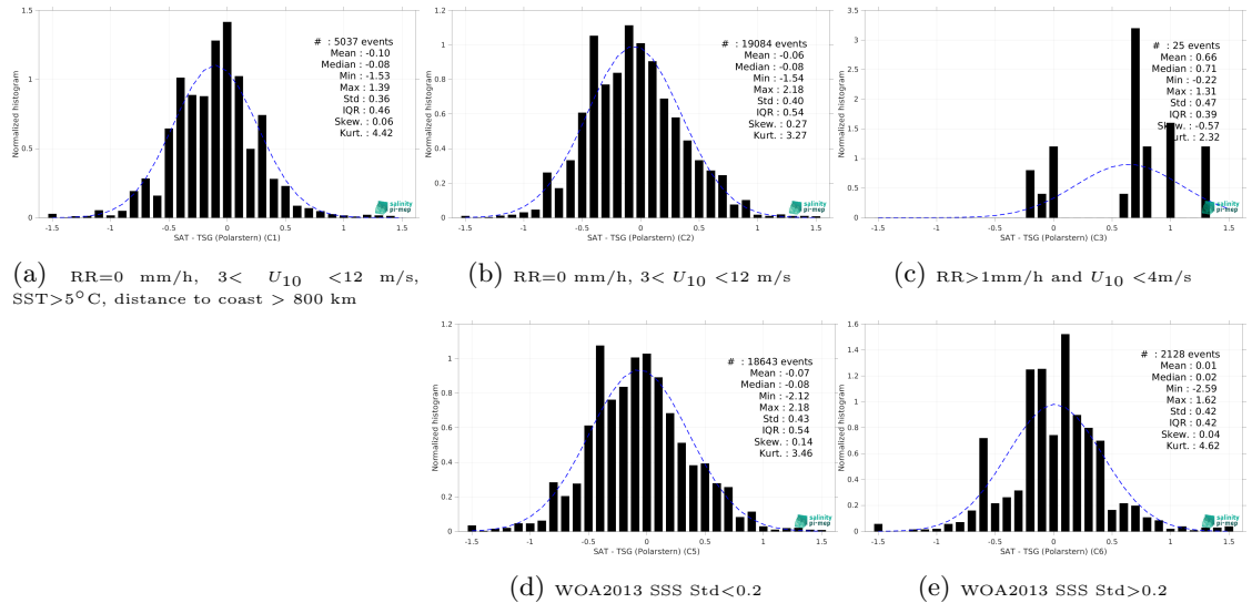
Figure 13: Normalized histogram of \Delta\text{SSS} (Aquarius SSS L2 CAP v5 (JPL) - TSG (Polarstern)) for 5 different subdatasets corresponding to: RR=0 mm/h, 3 < U_{10} < 12 m/s, SST >5^\circ\text{C} , distance to coast > 800 km (a), RR=0 mm/h, 3 < U_{10} < 12 m/s (b), RR >1 mm/h and U_{10} < 4 m/s (c), WOA2013 SSS Std <0.2 (d), WOA2013 SSS Std >0.2 (e).
