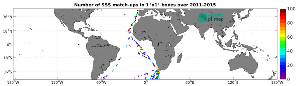
Figure 4: Number of SSS match-ups between TSG (Polarstern) SSS and the Aquarius SSS L2 CAP v5 (JPL) SSS product for the Mid-Low Latitudes 45N-45S Pi-MEP region over 1^\circ \times 1^\circ boxes and for the full satellite product period.
