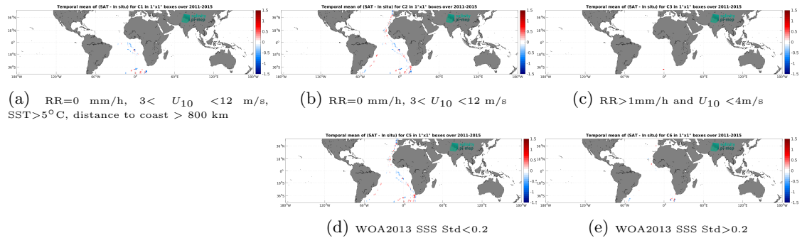
Figure 12: Temporal mean gridded over spatial boxes of size 1^\circ \times 1^\circ of \Delta\text{SSS} (Aquarius SSS L2 CAP v5 (JPL) - TSG (Polarstern)) for 5 different subdatasets corresponding to:RR=0 mm/h, 3 < U_{10} < 12 m/s, SST >5^\circ\text{C} , distance to coast > 800 km (a), RR=0 mm/h, 3 < U_{10} < 12 m/s (b), RR >1 mm/h and U_{10} < 4 m/s (c), WOA2013 SSS Std <0.2 (d), WOA2013 SSS Std >0.2 (e).
