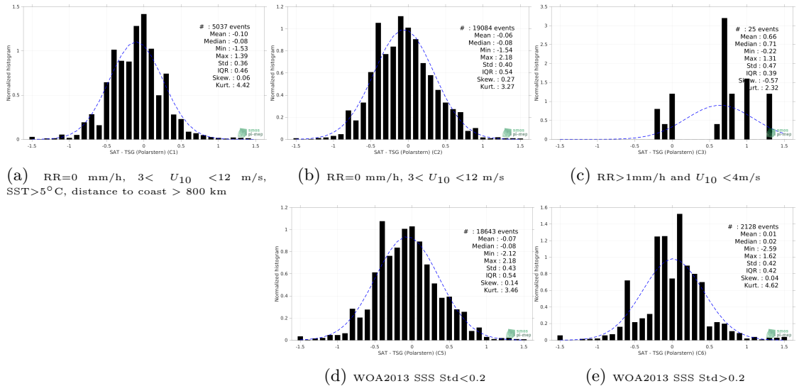
Figure 13: Normalized histogram of \Delta SSS (Aquarius SSS L2 CAP v5 (JPL) - TSG (Polarstern)) for 5 different subdatasets corresponding to: RR=0 mm/h, 3 < U_{10} < 12 m/s, SST >5^\circ\text{C} , distance to coast > 800 km (a), RR=0 mm/h, 3 < U_{10} < 12 m/s (b), RR >1 mm/h and U_{10} < 4 m/s (c), WOA2013 SSS Std <0.2 (d), WOA2013 SSS Std >0.2 (e).
