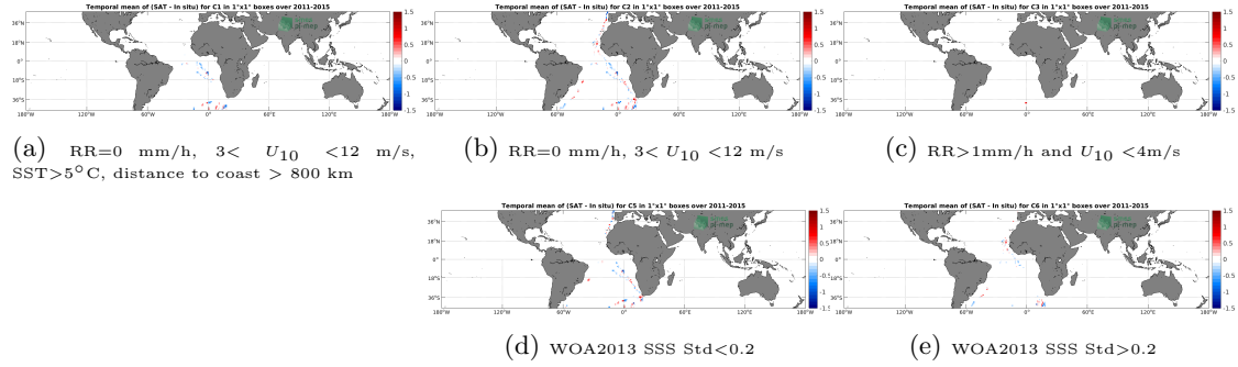
Figure 12: Temporal mean gridded over spatial boxes of size 1^\circ \times 1^\circ of \Delta SSS (Aquarius SSS L2 CAP v5 (JPL) - TSG (Polarstern)) for 5 different subdatasets corresponding to: RR=0 mm/h, 3 < U_{10} < 12 m/s, SST > 5^\circ C , distance to coast > 800 km (a), RR=0 mm/h, 3 < U_{10} < 12 m/s (b), RR > 1 mm/h and U_{10} < 4 m/s (c), WOA2013 SSS Std < 0.2 (d), WOA2013 SSS Std > 0.2 (e).
