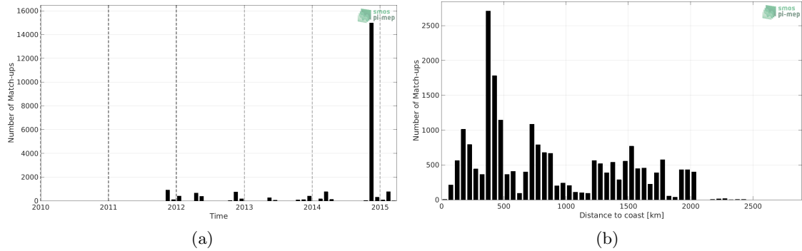
Figure 1: Number of match-ups between TSG (Polarstern) and Aquarius SSS L2 CAP v5 (JPL) SSS as a function of time (a) and as function of the distance to coast (b) over the Mid-Low Latitudes 45N-45S Pi-MEP region and for the full satellite product period.
