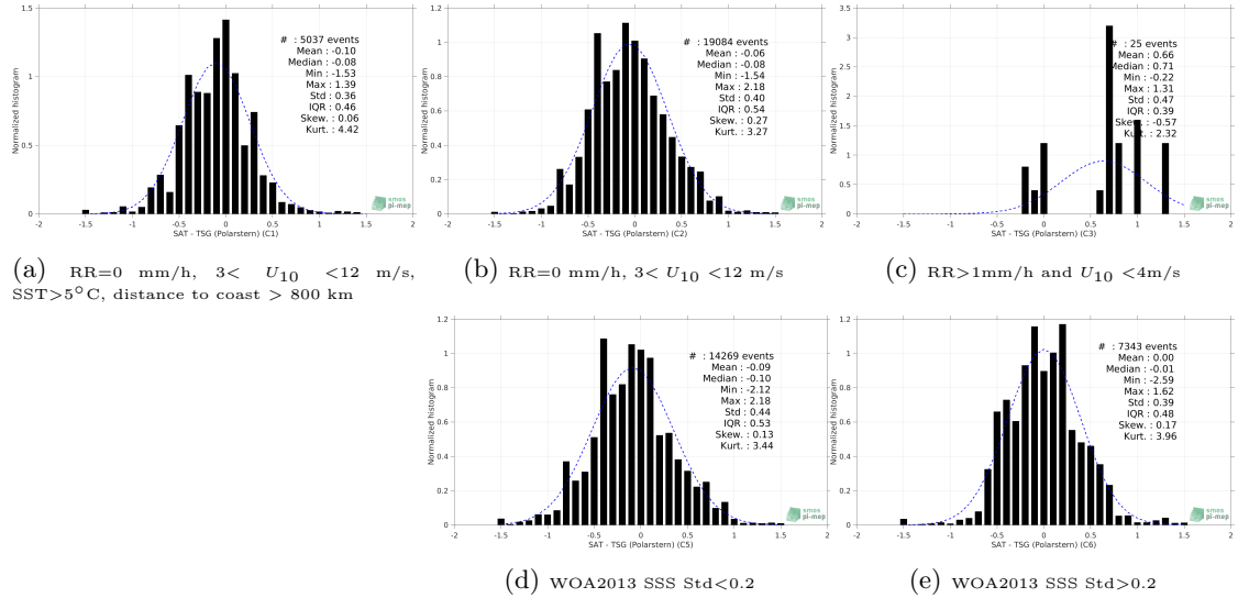
Figure 13: Normalized histogram of \Delta SSS (Aquarius SSS L2 CAP v5 (JPL) - TSG (Polarstern)) for 5 different subdatasets corresponding to: RR=0 mm/h, 3 < U_{10} < 12 m/s, SST > 5^\circ C , distance to coast > 800 km (a), RR=0 mm/h, 3 < U_{10} < 12 m/s (b), RR > 1 mm/h and U_{10} < 4 m/s (c), WOA2013 SSS Std < 0.2 (d), WOA2013 SSS Std > 0.2 (e).
