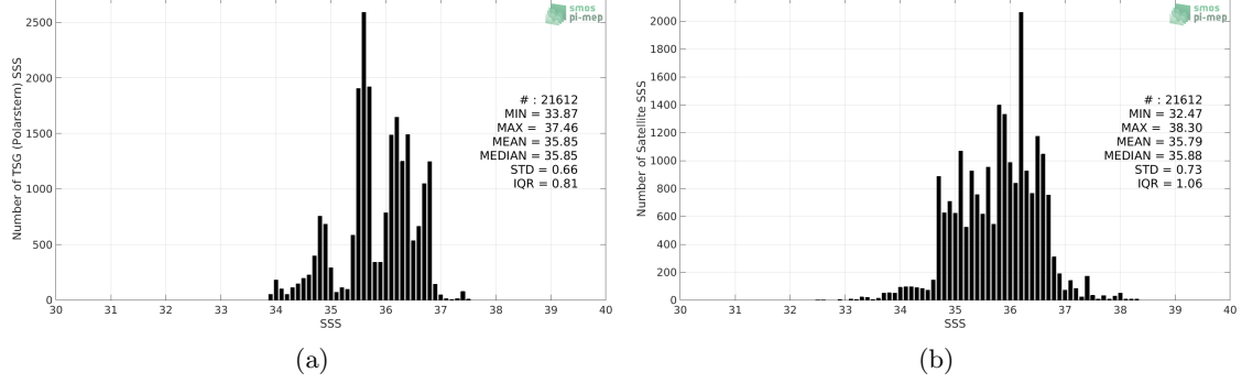
Figure 2: Histograms of SSS from TSG (Polarstern) (a) and Aquarius SSS L2 CAP v5 (JPL) (b) considering all match-up pairs per bins of 0.1 over the Mid-Low Latitudes 45N-45S Pi-MEP region and for the full satellite product period.
