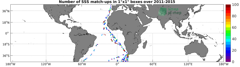
Figure 4: Number of SSS match-ups between TSG (Polarstern) SSS and the Aquarius SSS L2 CAP v5 (JPL) SSS product for the Mid-Low Latitudes 45N-45S Pi-MEP region over 1°x1° boxes and for the full satellite product period.
