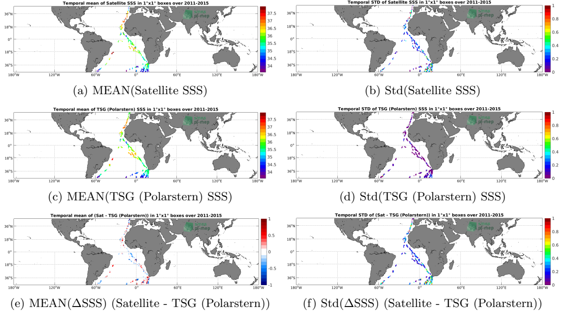
Figure 6: Temporal mean (left) and Std (right) of SSS from Aquarius SSS L2 CAP v5 (JPL) (top), TSG (Polarstern) (middle), and of \Delta SSS (Satellite - TSG (Polarstern)). Only match-up pairs are used to generate these maps.
