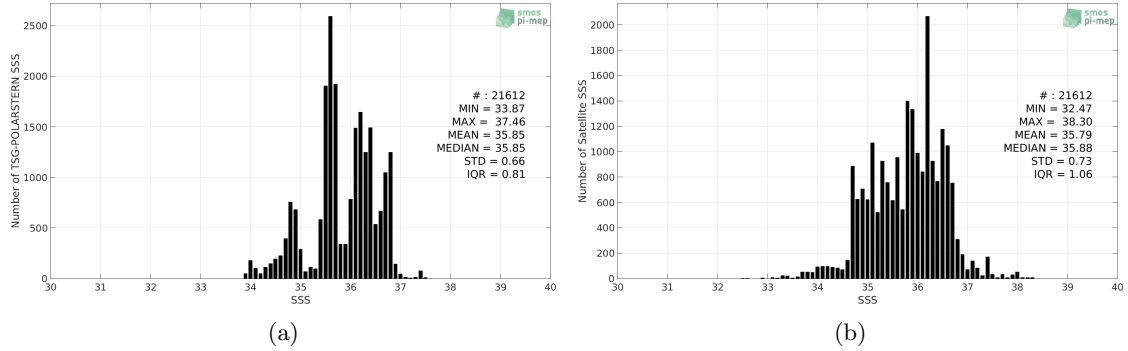
Figure 2: Histograms of SSS from TSG-POLARSTERN (a) and Aquarius-L2-JPL-V5 (b) considering all match-up pairs per bins of 0.1 over the Mid-Low Latitudes 45N-45S Pi-MEP region and for the full satellite product period.
