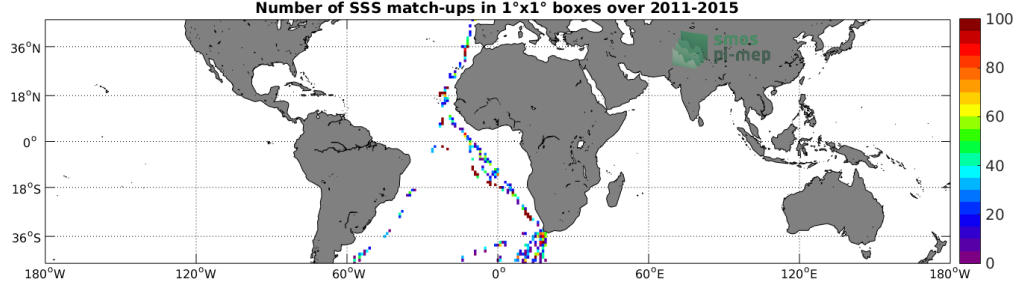
Figure 4: Number of SSS match-ups between TSG-POLARSTERN SSS and the Aquarius-L2-JPL-V5 SSS product for the Mid-Low Latitudes 45N-45S Pi-MEP region over 1^\circ \times 1^\circ boxes and for the full satellite product period.
