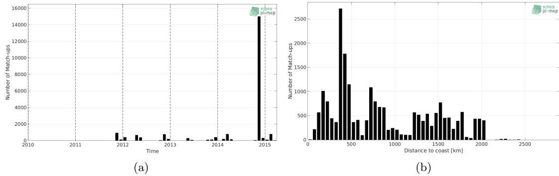
Figure 1: Number of match-ups between TSG-POLARSTERN and Aquarius-L2-JPL-V5 SSS as a function of time (a) and as function of the distance to coast (b) over the Mid-Low Latitudes 45N-45S Pi-MEP region and for the full satellite product period.
