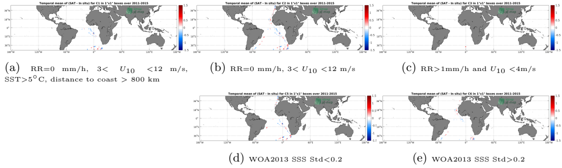
Figure 12: Temporal mean gridded over spatial boxes of size 1^\circ \times 1^\circ of \Delta SSS (Aquarius-L2-JPL-V5 - TSG-POLARSTERN) for 5 different subdatasets corresponding to: RR=0 mm/h, 3 < U_{10} < 12 m/s, SST > 5^\circ C , distance to coast > 800 km (a), RR=0 mm/h, 3 < U_{10} < 12 m/s (b), RR > 1 mm/h and U_{10} < 4 m/s (c), WOA2013 SSS Std < 0.2 (d), WOA2013 SSS Std > 0.2 (e).
