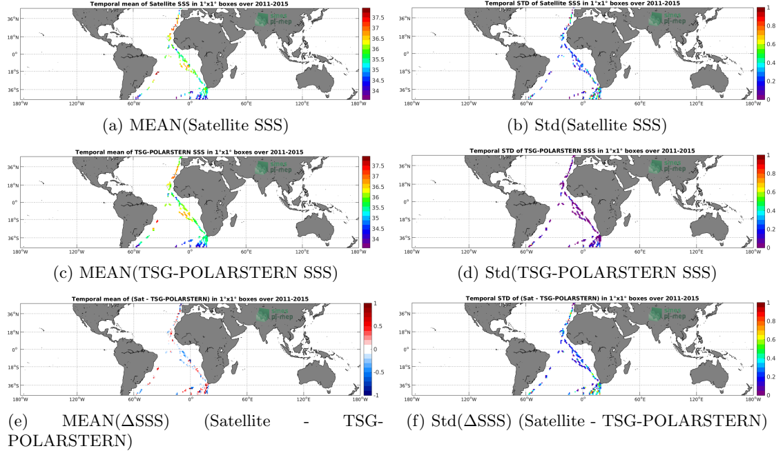
Figure 6: Temporal mean (left) and Std (right) of SSS from Aquarius-L2-JPL-V5 (top), TSG-POLARSTERN (middle), and of \Delta SSS (Satellite - TSG-POLARSTERN). Only match-up pairs are used to generate these maps.
