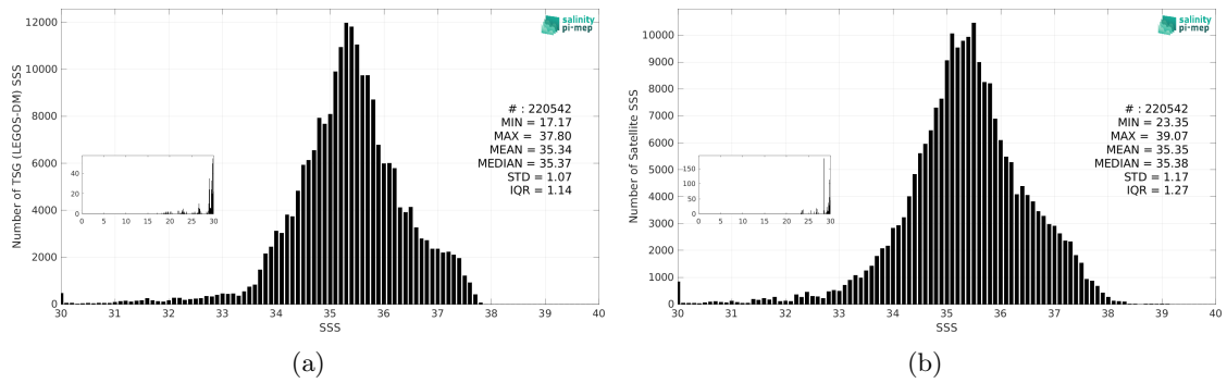
Figure 3: Histograms of SSS from TSG (LEGOS-DM) (a) and Aquarius SSS L2 CAP v5 (JPL) (b) considering all match-up pairs per bins of 0.1 over the Mid-Low Latitudes 45N-45S Pi-MEP region and for the full satellite product period.
