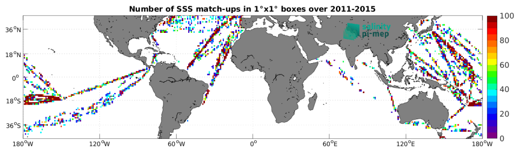
Figure 5: Number of SSS match-ups between TSG (LEGOS-DM) SSS and the Aquarius SSS L2 CAP v5 (JPL) SSS product for the Mid-Low Latitudes 45N-45S Pi-MEP region over 1^\circ \times 1^\circ boxes and for the full satellite product period.
