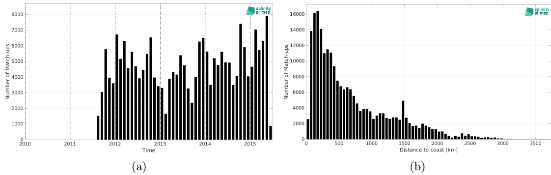
Figure 2: Number of match-ups between TSG (LEGOS-DM) and Aquarius SSS L2 CAP v5 (JPL) SSS as a function of time (a) and as function of the distance to coast (b) over the Mid-Low Latitudes 45N-45S Pi-MEP region and for the full satellite product period.
