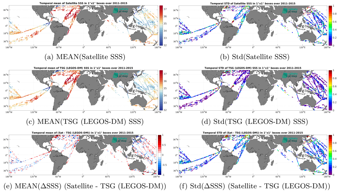
Figure 7: Temporal mean (left) and Std (right) of SSS from Aquarius SSS L2 CAP v5 (JPL) (top), TSG (LEGOS-DM) (middle), and of \Delta SSS (Satellite - TSG (LEGOS-DM)). Only match-up pairs are used to generate these maps.
