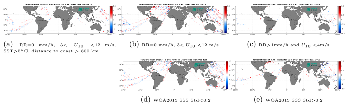
Figure 14: Temporal mean gridded over spatial boxes of size 1^\circ \times 1^\circ of \Delta\text{SSS} (Aquarius SSS L2 CAP v5 (JPL) - TSG (LEGOS-DM)) for 5 different subdatasets corresponding to: RR=0 mm/h, 3 < U_{10} < 12 m/s, SST > 5°C, distance to coast > 800 km (a), RR=0 mm/h, 3 < U_{10} < 12 m/s (b), RR > 1mm/h and U_{10} < 4 m/s (c), WOA2013 SSS Std < 0.2 (d), WOA2013 SSS Std > 0.2 (e).
