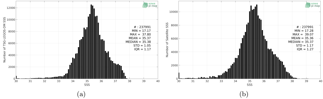
Figure 2: Histograms of SSS from TSG-LEGOS-DM (a) and Aquarius-L2-JPL-V5 (b) considering all match-up pairs per bins of 0.1 over the Mid-Low Latitudes 45N-45S Pi-MEP region and for the full satellite product period.
