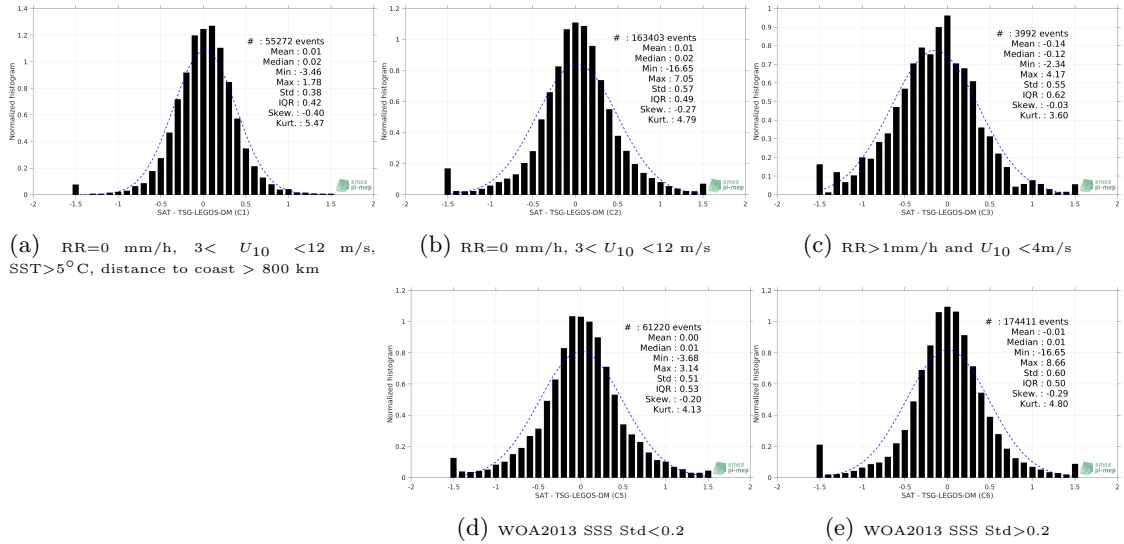
Figure 13: Normalized histogram of \Delta SSS (Aquarius-L2-JPL-V5 - TSG-LEGOS-DM) for 5 different subdatasets corresponding to: RR=0 mm/h, 3 < U_{10} < 12 m/s, SST > 5^\circ\text{C} , distance to coast > 800 km (a), RR=0 mm/h, 3 < U_{10} < 12 m/s (b), RR > 1\text{mm/h} and U_{10} < 4\text{m/s} (c), WOA2013 SSS Std < 0.2 (d), WOA2013 SSS Std > 0.2 (e).
