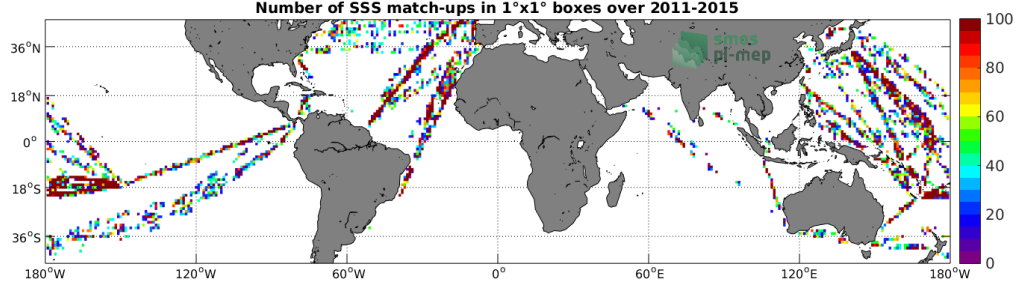
Figure 4: Number of SSS match-ups between TSG-LEGOS-DM SSS and the Aquarius-L2-JPL-V5 SSS product for the Mid-Low Latitudes 45N-45S Pi-MEP region over 1^\circ \times 1^\circ boxes and for the full satellite product period.
