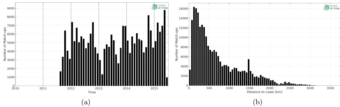
Figure 1: Number of match-ups between TSG-LEGOS-DM and Aquarius-L2-JPL-V5 SSS as a function of time (a) and as function of the distance to coast (b) over the Mid-Low Latitudes 45N-45S Pi-MEP region and for the full satellite product period.
