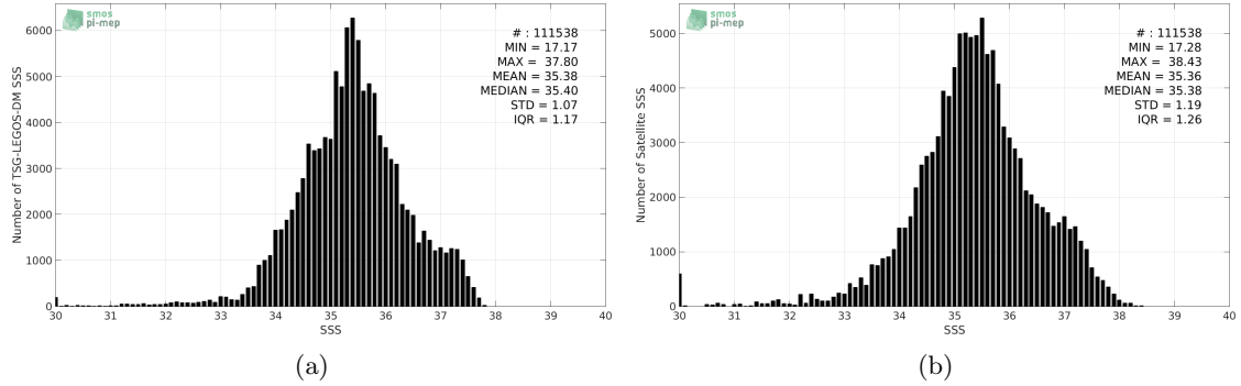
Figure 2: Histograms of SSS from TSG-LEGOS-DM (a) and Aquarius-L2-JPL-V5 (b) considering all match-up pairs per bins of 0.1 over the Mid-Low Latitudes 45N-45S Pi-MEP region and for the full satellite product period.
