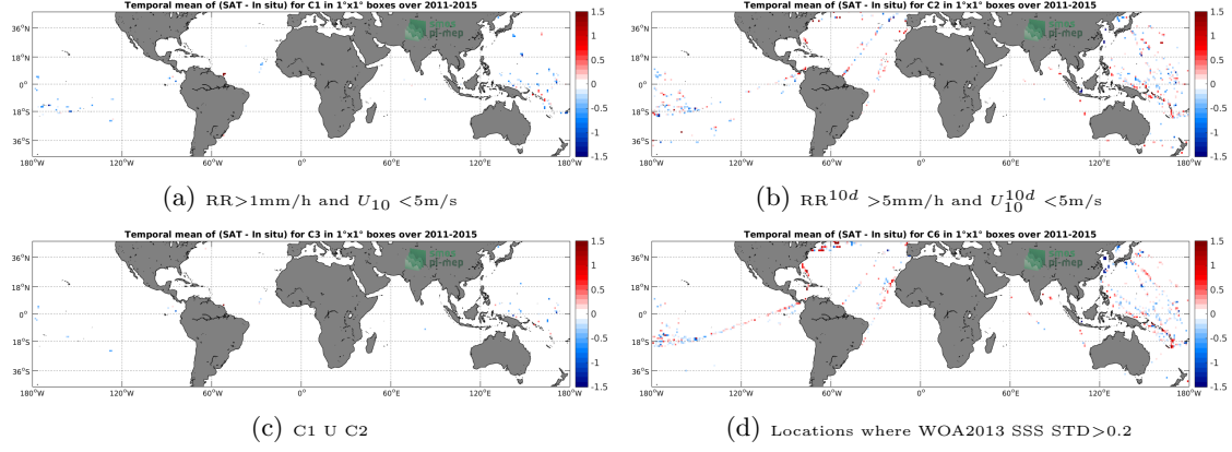
Figure 12: Temporal mean gridded over spatial boxes of size 1^\circ \times 1^\circ of \Delta SSS (Aquarius-L2-JPL-V5 - TSG-LEGOS-DM) for 4 different subdatasets corresponding to: RR > 1\text{mm/h} and U_{10} < 5\text{m/s} (a), RR^{10d} > 5\text{mm/h} and U_{10}^{10d} < 5\text{m/s} (b), C1 U C2 (c), Locations where WOA2013 SSS STD > 0.2 (d).
