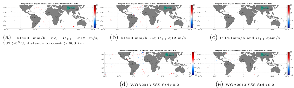
Figure 12: Temporal mean gridded over spatial boxes of size 1^\circ \times 1^\circ of \Delta\text{SSS} (Aquarius SSS L2 CAP v5 (JPL) - TSG (GOSUD-Sailing-ship)) for 5 different subdatasets corresponding to: RR=0 mm/h, 3 < U_{10} < 12 m/s, SST > 5°C, distance to coast > 800 km (a), RR=0 mm/h, 3 < U_{10} < 12 m/s (b), RR > 1mm/h and U_{10} < 4 m/s (c), WOA2013 SSS Std < 0.2 (d), WOA2013 SSS Std > 0.2 (e).
