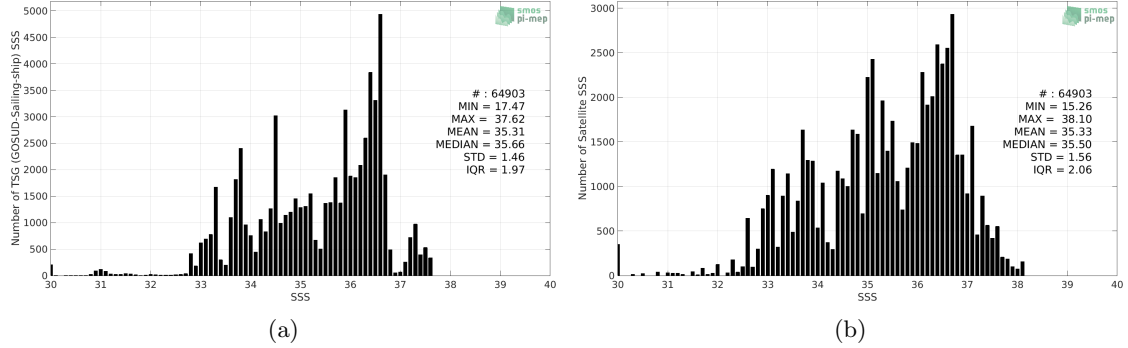
Figure 2: Histograms of SSS from TSG (GOSUD-Sailing-ship) (a) and Aquarius SSS L2 CAP v5 (JPL) (b) considering all match-up pairs per bins of 0.1 over the Mid-Low Latitudes 45N-45S Pi-MEP region and for the full satellite product period.
