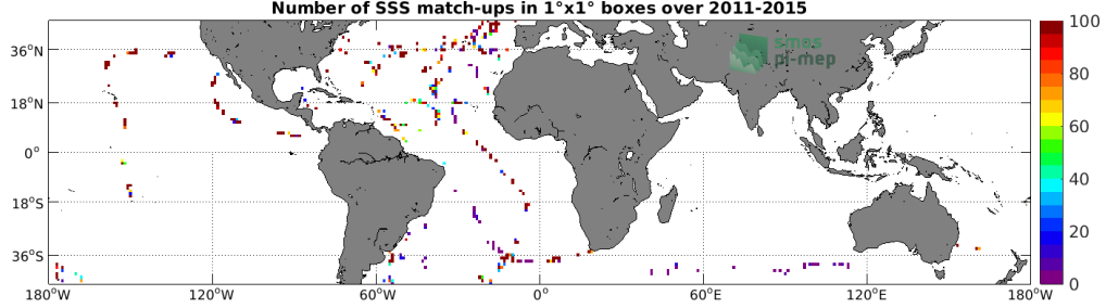
Figure 4: Number of SSS match-ups between TSG (GOSUD-Sailing-ship) SSS and the Aquarius SSS L2 CAP v5 (JPL) SSS product for the Mid-Low Latitudes 45N-45S Pi-MEP region over 1°x1° boxes and for the full satellite product period.
