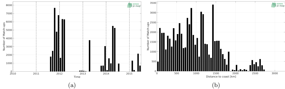
Figure 1: Number of match-ups between TSG-GOSUD-Sailing-ship and Aquarius-L2-JPL-V5 SSS as a function of time (a) and as function of the distance to coast (b) over the Mid-Low Latitudes 45N-45S Pi-MEP region and for the full satellite product period.
