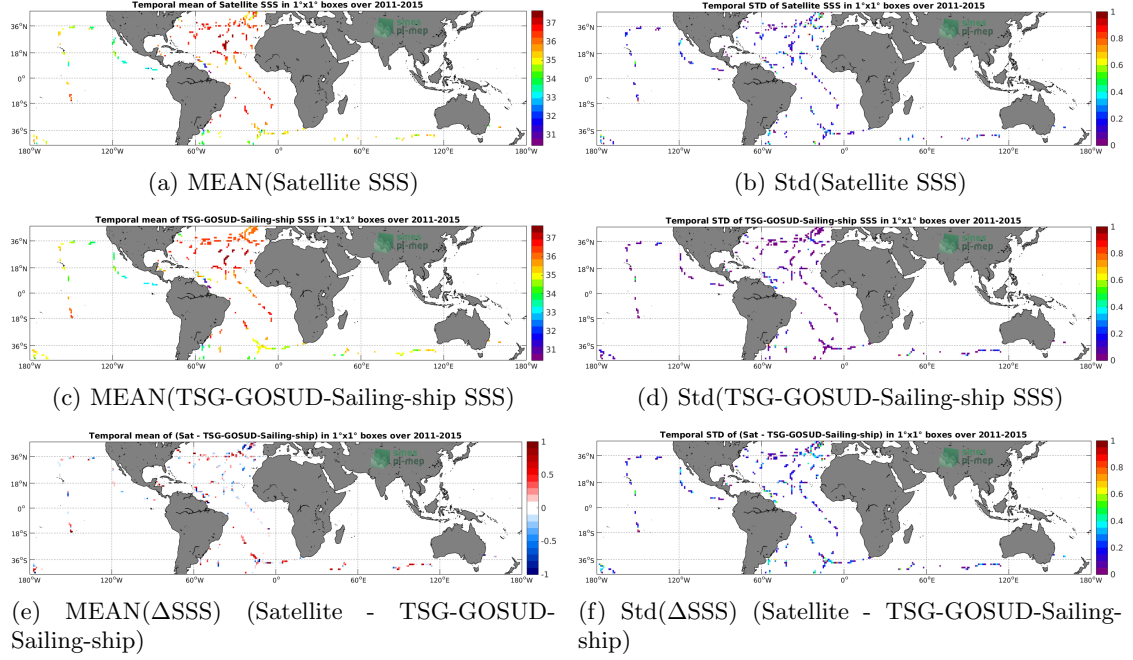
Figure 6: Temporal mean (left) and Std (right) of SSS from Aquarius-L2-JPL-V5 (top), TSG-GOSUD-Sailing-ship (middle), and of \Delta SSS (Satellite - TSG-GOSUD-Sailing-ship). Only match-up pairs are used to generate these maps.
