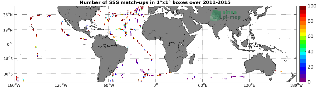
Figure 4: Number of SSS match-ups between TSG-GOSUD-Sailing-ship SSS and the Aquarius-L2-JPL-V5 SSS product for the Mid-Low Latitudes 45N-45S Pi-MEP region over 1^\circ \times 1^\circ boxes and for the full satellite product period.
