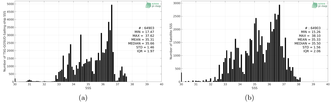
Figure 2: Histograms of SSS from TSG-GOSUD-Sailing-ship (a) and Aquarius-L2-JPL-V5 (b) considering all match-up pairs per bins of 0.1 over the Mid-Low Latitudes 45N-45S Pi-MEP region and for the full satellite product period.
