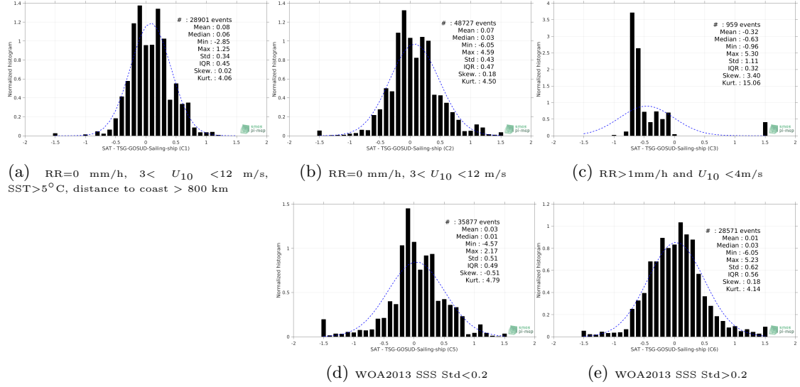
Figure 13: Normalized histogram of \Delta SSS (Aquarius-L2-JPL-V5 - TSG-GOSUD-Sailing-ship) for 5 different subdatasets corresponding to: RR=0 mm/h, 3 < U_{10} < 12 m/s, SST > 5^\circ\text{C} , distance to coast > 800 km (a), RR=0 mm/h, 3 < U_{10} < 12 m/s (b), RR > 1 mm/h and U_{10} < 4 m/s (c), WOA2013 SSS Std < 0.2 (d), WOA2013 SSS Std > 0.2 (e).
