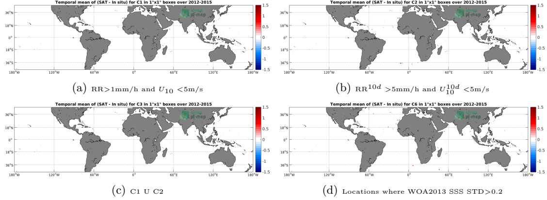
Figure 12: Temporal mean gridded over spatial boxes of size 1^\circ \times 1^\circ of \Delta SSS (Aquarius-L2-JPL-V5 - TSG-GOSUD-Sailing-ship) for 4 different subdatasets corresponding to: RR > 1mm/h and U_{10} < 5\text{m/s} (a), RR^{10d} > 5\text{mm/h} and U_{10d} < 5\text{m/s} (b), C1 U C2 (c), Locations where WOA2013 SSS STD > 0.2 (d).
