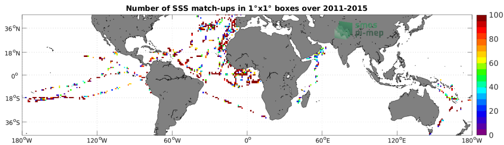
Figure 4: Number of SSS match-ups between TSG (GOSUD-Research-vessel) SSS and the Aquarius SSS L2 CAP v5 (JPL) SSS product for the Mid-Low Latitudes 45N-45S Pi-MEP region over 1^\circ \times 1^\circ boxes and for the full satellite product period.
