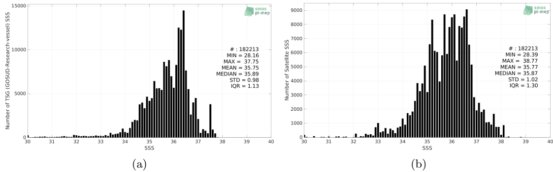
Figure 2: Histograms of SSS from TSG (GOSUD-Research-vessel) (a) and Aquarius SSS L2 CAP v5 (JPL) (b) considering all match-up pairs per bins of 0.1 over the Mid-Low Latitudes 45N-45S Pi-MEP region and for the full satellite product period.
