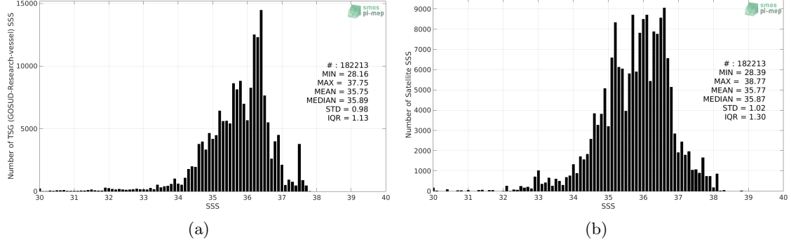
Figure 2: Histograms of SSS from TSG (GOSUD-Research-vessel) (a) and Aquarius SSS L2 CAP v5 (JPL) (b) considering all match-up pairs per bins of 0.1 over the Mid-Low Latitudes 45N-45S Pi-MEP region and for the full satellite product period.
