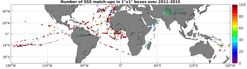
Figure 4: Number of SSS match-ups between TSG (GOSUD-Research-vessel) SSS and the Aquarius SSS L2 CAP v5 (JPL) SSS product for the Mid-Low Latitudes 45N-45S Pi-MEP region over 1°x1° boxes and for the full satellite product period.
