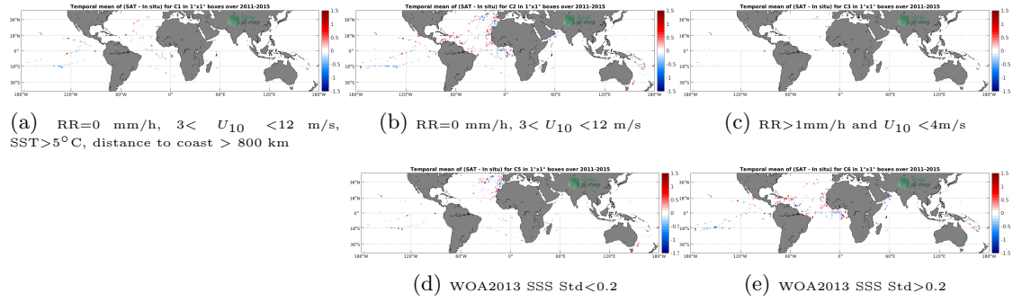
Figure 12: Temporal mean gridded over spatial boxes of size 1^\circ \times 1^\circ of \Delta SSS (Aquarius SSS L2 CAP v5 (JPL) - TSG (GOSUD-Research-vessel)) for 5 different subdatasets corresponding to: RR=0 mm/h, 3 < U_{10} < 12 m/s, SST > 5^\circ C , distance to coast > 800 km (a), RR=0 mm/h, 3 < U_{10} < 12 m/s (b), RR > 1 mm/h and U_{10} < 4 m/s (c), WOA2013 SSS Std < 0.2 (d), WOA2013 SSS Std > 0.2 (e).
