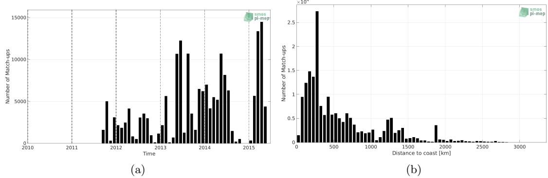
Figure 1: Number of match-ups between TSG (GOSUD-Research-vessel) and Aquarius SSS L2 CAP v5 (JPL) SSS as a function of time (a) and as function of the distance to coast (b) over the Mid-Low Latitudes 45N-45S Pi-MEP region and for the full satellite product period.
