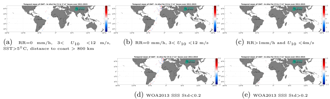
Figure 14: Temporal mean gridded over spatial boxes of size 1^\circ \times 1^\circ of \Delta\text{SSS} (Aquarius SSS L2 CAP v5 (JPL) - TSG (CSIC-UTM)) for 5 different subdatasets corresponding to: RR=0 mm/h, 3 < U_{10} < 12 m/s, SST > 5°C, distance to coast > 800 km (a), RR=0 mm/h, 3 < U_{10} < 12 m/s (b), RR > 1mm/h and U_{10} < 4 m/s (c), WOA2013 SSS Std < 0.2 (d), WOA2013 SSS Std > 0.2 (e).
