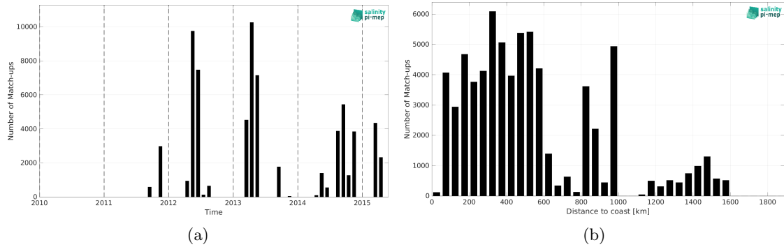
Figure 2: Number of match-ups between TSG (CSIC-UTM) and Aquarius SSS L2 CAP v5 (JPL) SSS as a function of time (a) and as function of the distance to coast (b) over the Mid-Low Latitudes 45N-45S Pi-MEP region and for the full satellite product period.
