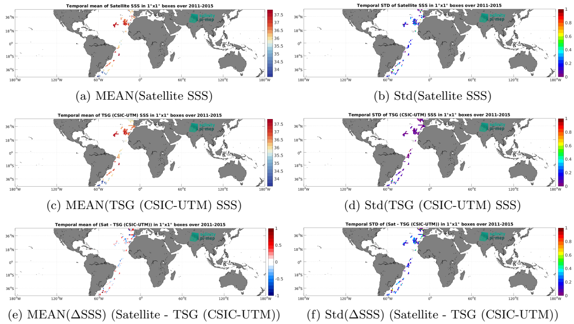
Figure 7: Temporal mean (left) and Std (right) of SSS from Aquarius SSS L2 CAP v5 (JPL) (top), TSG (CSIC-UTM) (middle), and of \Delta SSS (Satellite - TSG (CSIC-UTM)). Only match-up pairs are used to generate these maps.
