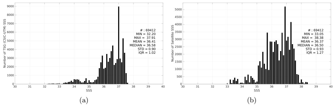
Figure 3: Histograms of SSS from TSG (CSIC-UTM) (a) and Aquarius SSS L2 CAP v5 (JPL) (b) considering all match-up pairs per bins of 0.1 over the Mid-Low Latitudes 45N-45S Pi-MEP region and for the full satellite product period.
