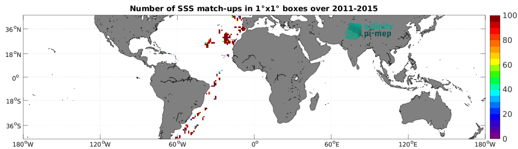
Figure 5: Number of SSS match-ups between TSG (CSIC-UTM) SSS and the Aquarius SSS L2 CAP v5 (JPL) SSS product for the Mid-Low Latitudes 45N-45S Pi-MEP region over 1^\circ \times 1^\circ boxes and for the full satellite product period.
