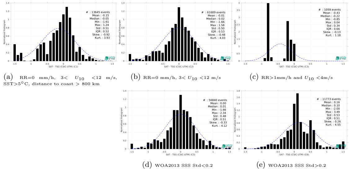
Figure 13: Normalized histogram of \Delta SSS (Aquarius SSS L2 CAP v5 (JPL) - TSG (CSIC-UTM)) for 5 different subdatasets corresponding to: RR=0 mm/h, 3 < U_{10} < 12 m/s, SST >5^\circ\text{C} , distance to coast > 800 km (a), RR=0 mm/h, 3 < U_{10} < 12 m/s (b), RR >1 mm/h and U_{10} < 4 m/s (c), WOA2013 SSS Std <0.2 (d), WOA2013 SSS Std >0.2 (e).
