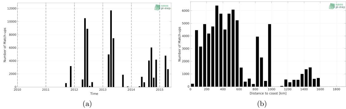
Figure 1: Number of match-ups between TSG (CSIC-UTM) and Aquarius SSS L2 CAP v5 (JPL) SSS as a function of time (a) and as function of the distance to coast (b) over the Mid-Low Latitudes 45N-45S Pi-MEP region and for the full satellite product period.
