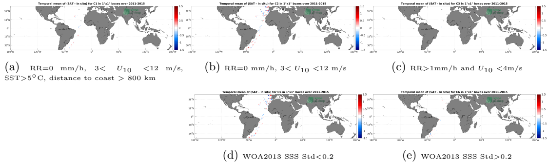
Figure 12: Temporal mean gridded over spatial boxes of size 1^\circ \times 1^\circ of \Delta SSS (Aquarius SSS L2 CAP v5 (JPL) - TSG (CSIC-UTM)) for 5 different subdatasets corresponding to: RR=0 mm/h, 3 < U_{10} < 12 m/s, SST>5°C, distance to coast > 800 km (a), RR=0 mm/h, 3 < U_{10} < 12 m/s (b), RR>1mm/h and U_{10} < 4 m/s (c), WOA2013 SSS Std<0.2 (d), WOA2013 SSS Std>0.2 (e).
