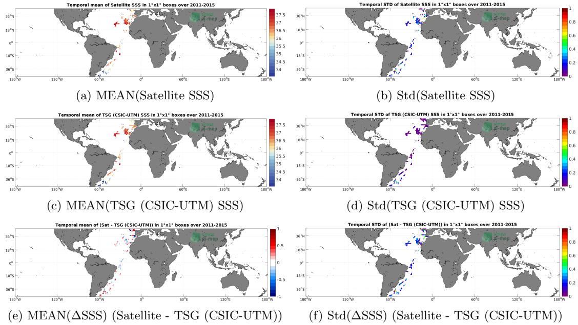
Figure 6: Temporal mean (left) and Std (right) of SSS from Aquarius SSS L2 CAP v5 (JPL) (top), TSG (CSIC-UTM) (middle), and of \Delta SSS (Satellite - TSG (CSIC-UTM)). Only match-up pairs are used to generate these maps.
