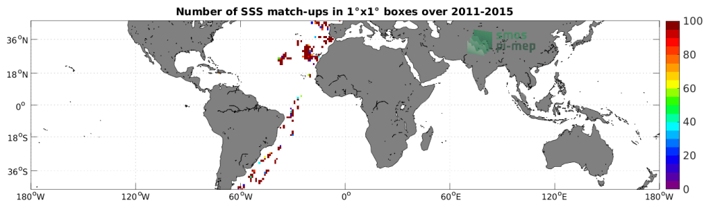
Figure 4: Number of SSS match-ups between TSG (CSIC-UTM) SSS and the Aquarius SSS L2 CAP v5 (JPL) SSS product for the Mid-Low Latitudes 45N-45S Pi-MEP region over 1^\circ \times 1^\circ boxes and for the full satellite product period.
