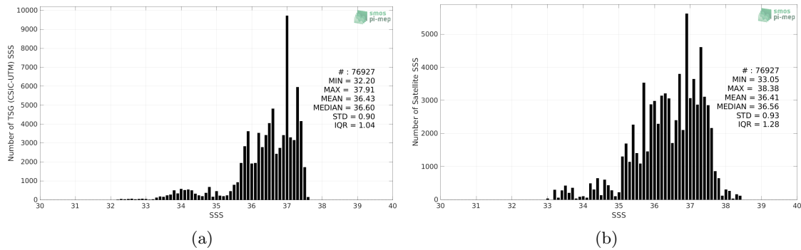
Figure 2: Histograms of SSS from TSG (CSIC-UTM) (a) and Aquarius SSS L2 CAP v5 (JPL) (b) considering all match-up pairs per bins of 0.1 over the Mid-Low Latitudes 45N-45S Pi-MEP region and for the full satellite product period.
