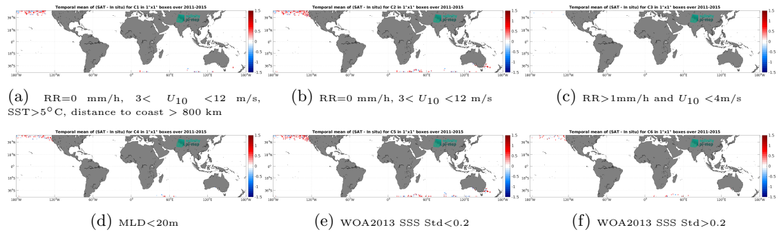
Figure 14: Temporal mean gridded over spatial boxes of size 1^\circ \times 1^\circ of \Delta\text{SSS} (Aquarius SSS L2 CAP v5 (JPL) - Marine mammals) for 6 different subdatasets corresponding to:RR=0 mm/h, 3 < U_{10} < 12 m/s, SST>5°C, distance to coast > 800 km (a), RR=0 mm/h, 3 < U_{10} < 12 m/s (b), RR>1mm/h and U_{10} < 4 m/s (c),MLD<20m (d),WOA2013 SSS Std<0.2 (e),WOA2013 SSS Std>0.2 (f).
