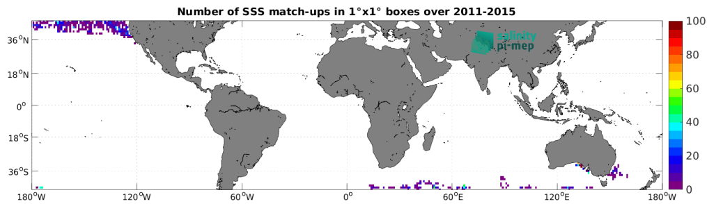
Figure 5: Number of SSS match-ups between Marine mammals SSS and the Aquarius SSS L2 CAP v5 (JPL) SSS product for the Mid-Low Latitudes 45N-45S Pi-MEP region over 1^\circ \times 1^\circ boxes and for the full satellite product period.
