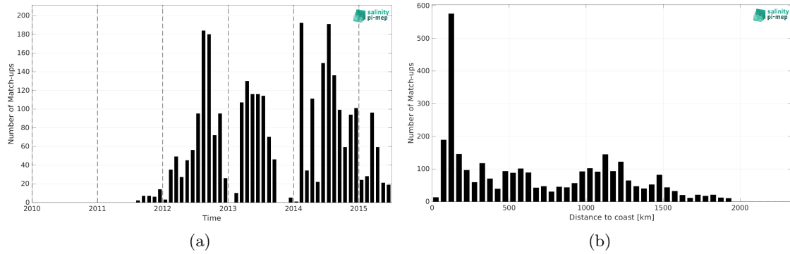
Figure 2: Number of match-ups between Marine mammals and Aquarius SSS L2 CAP v5 (JPL) SSS as a function of time (a) and as function of the distance to coast (b) over the Mid-Low Latitudes 45N-45S Pi-MEP region and for the full satellite product period.
