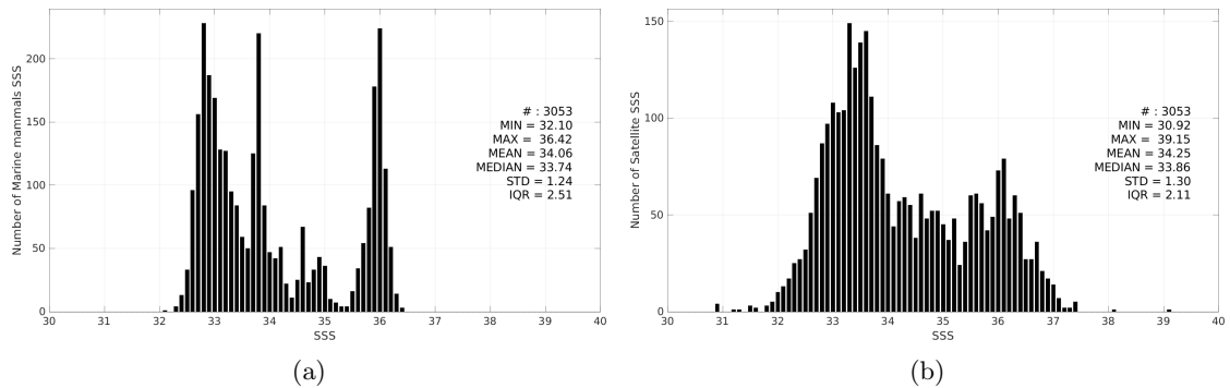
Figure 3: Histograms of SSS from Marine mammals (a) and Aquarius SSS L2 CAP v5 (JPL) (b) considering all match-up pairs per bins of 0.1 over the Mid-Low Latitudes 45N-45S Pi-MEP region and for the full satellite product period.
