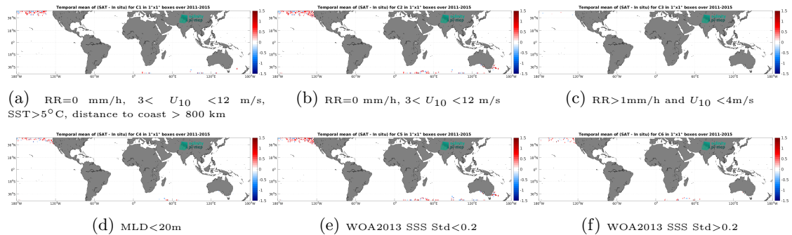
Figure 14: Temporal mean gridded over spatial boxes of size 1^\circ \times 1^\circ of \Delta SSS (Aquarius SSS L2 CAP v5 (JPL) - Marine mammals) for 6 different subdatasets corresponding to: RR=0 mm/h, 3 < U_{10} < 12 m/s, SST > 5°C, distance to coast > 800 km (a), RR=0 mm/h, 3 < U_{10} < 12 m/s (b), RR > 1mm/h and U_{10} < 4 m/s (c), MLD < 20m (d), WOA2013 SSS Std < 0.2 (e), WOA2013 SSS Std > 0.2 (f).
