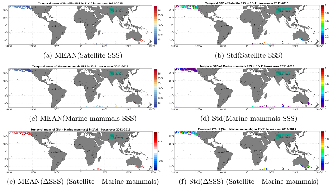
Figure 7: Temporal mean (left) and Std (right) of SSS from Aquarius SSS L2 CAP v5 (JPL) (top), Marine mammals (middle), and of \Delta SSS (Satellite - Marine mammals). Only match-up pairs are used to generate these maps.
