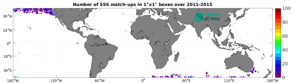
Figure 4: Number of SSS match-ups between Marine mammals SSS and the Aquarius SSS L2 CAP v5 (JPL) SSS product for the Mid-Low Latitudes 45N-45S Pi-MEP region over 1^\circ \times 1^\circ boxes and for the full satellite product period.
