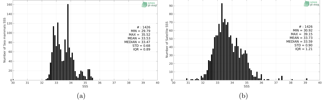
Figure 2: Histograms of SSS from Sea mammals (a) and Aquarius SSS L2 CAP v5 (JPL) (b) considering all match-up pairs per bins of 0.1 over the Mid-Low Latitudes 45N-45S Pi-MEP region and for the full satellite product period.
