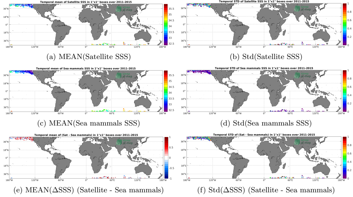
Figure 6: Temporal mean (left) and Std (right) of SSS from Aquarius SSS L2 CAP v5 (JPL) (top), Sea mammals (middle), and of \Delta SSS (Satellite - Sea mammals). Only match-up pairs are used to generate these maps.
