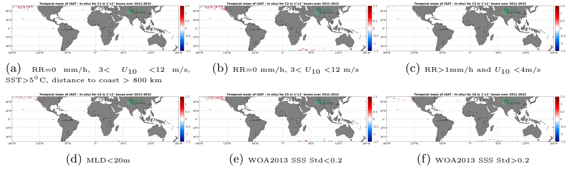
Figure 12: Temporal mean gridded over spatial boxes of size 1^\circ \times 1^\circ of \Delta SSS (Aquarius SSS L2 CAP v5 (JPL) - Sea mammals) for 6 different subdatasets corresponding to: RR=0 mm/h, 3 < U_{10} < 12 m/s, SST > 5^\circ C , distance to coast > 800 km (a), RR=0 mm/h, 3 < U_{10} < 12 m/s (b), RR > 1 mm/h and U_{10} < 4 m/s (c), MLD < 20 m (d), WOA2013 SSS Std < 0.2 (e), WOA2013 SSS Std > 0.2 (f).
