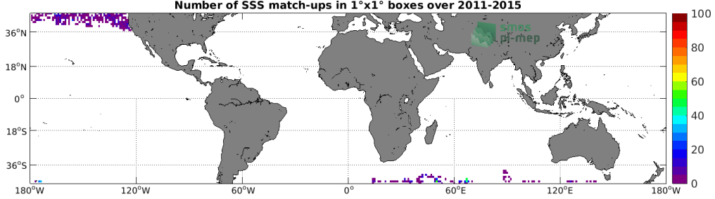
Figure 4: Number of SSS match-ups between Sea mammals SSS and the Aquarius SSS L2 CAP v5 (JPL) SSS product for the Mid-Low Latitudes 45N-45S Pi-MEP region over 1°x1° boxes and for the full satellite product period.
