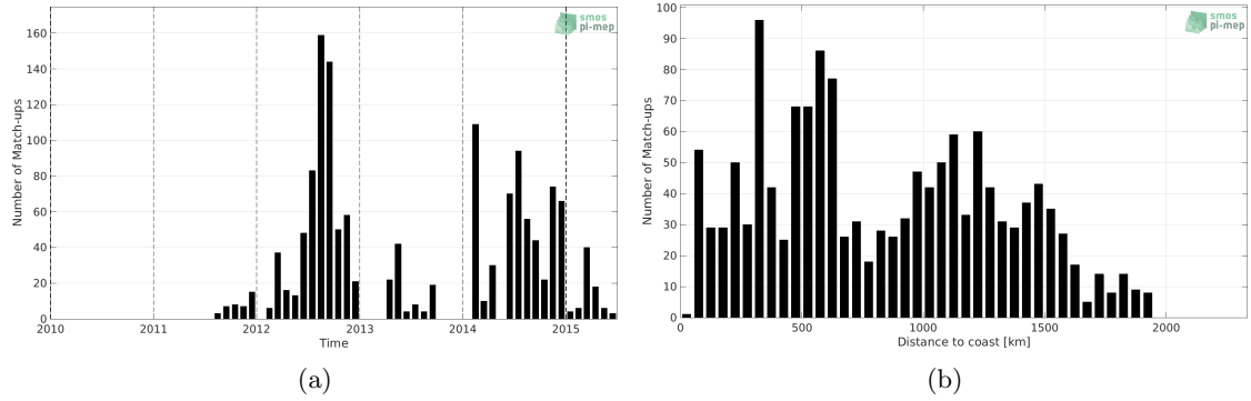
Figure 1: Number of match-ups between Sea mammals and Aquarius SSS L2 CAP v5 (JPL) SSS as a function of time (a) and as function of the distance to coast (b) over the Mid-Low Latitudes 45N-45S Pi-MEP region and for the full satellite product period.
