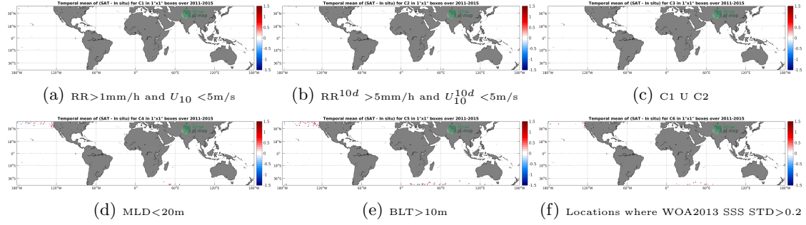
Figure 12: Temporal mean gridded over spatial boxes of size 1^\circ \times 1^\circ of \Delta\text{SSS} (Aquarius-L2-JPL-V5 - Sea mammals) for 6 different subdatasets corresponding to: RR>1\text{mm/h} and U_{10}<5\text{m/s} (a), RR^{10d}>5\text{mm/h} and U_{10}^{10d}<5\text{m/s} (b), C1 U C2 (c), MLD<20\text{m} (d), BLT>10\text{m} (e), Locations where WOA2013 SSS STD >0.2 (f).
