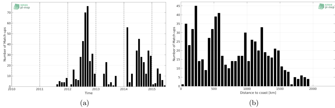
Figure 1: Number of match-ups between Sea mammals and Aquarius-L2-JPL-V5 SSS as a function of time (a) and as function of the distance to coast (b) over the Mid-Low Latitudes 45N-45S Pi-MEP region and for the full satellite product period.
