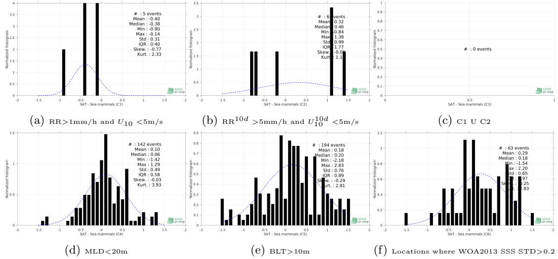
Figure 13: Normalized histogram of \Delta\text{SSS} (Aquarius-L2-JPL-V5 - Sea mammals) for 6 different subdatasets corresponding to: RR>1\text{mm/h} and U_{10}<5\text{m/s} (a), RR^{10d}>5\text{mm/h} and U_{10}^{10d}<5\text{m/s} (b), C1 U C2 (c), MLD<20\text{m} (d), BLT>10\text{m} (e), Locations where WOA2013 SSS STD >0.2 (f).
