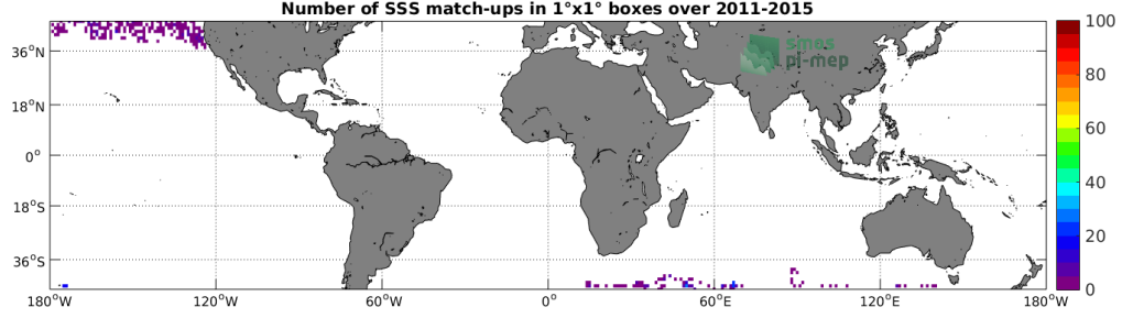
Figure 4: Number of SSS match-ups between Sea mammals SSS and the Aquarius-L2-JPL-V5 SSS product for the Mid-Low Latitudes 45N-45S Pi-MEP region over 1°x1° boxes and for the full satellite product period.
