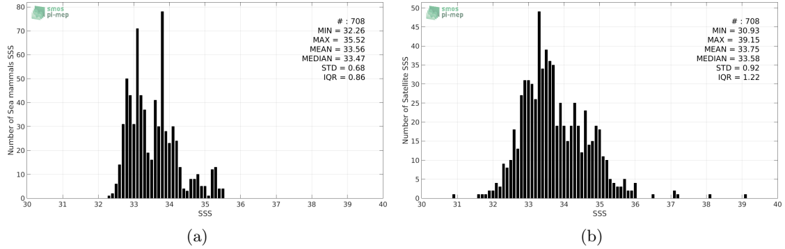
Figure 2: Histograms of SSS from Sea mammals (a) and Aquarius-L2-JPL-V5 (b) considering all match-up pairs per bins of 0.1 over the Mid-Low Latitudes 45N-45S Pi-MEP region and for the full satellite product period.
