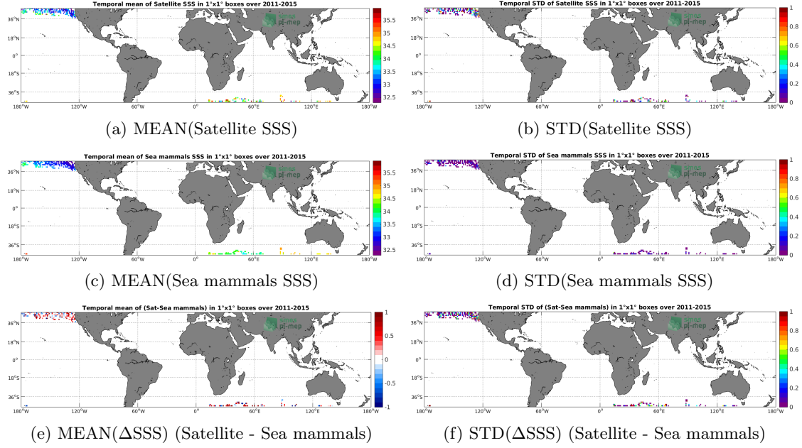
Figure 6: Temporal mean (left) and STD (right) of SSS from Aquarius-L2-JPL-V5 (top), Sea mammals (middle), and of \Delta SSS (Satellite - Sea mammals). Only match-up pairs are used to generate these maps.
