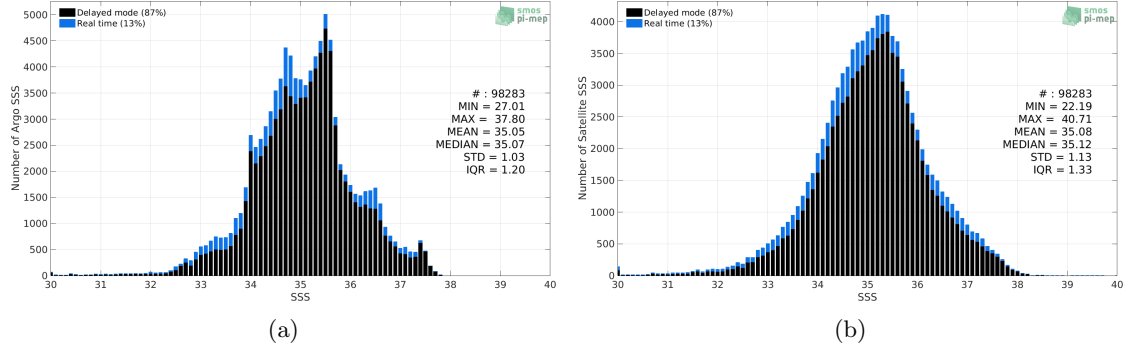
Figure 2: Histograms of SSS from Argo (a) and Aquarius SSS L2 CAP v5 (JPL) (b) considering all match-up pairs per bins of 0.1 over the Mid-Low Latitudes 45N-45S Pi-MEP region and for the full satellite product period.
