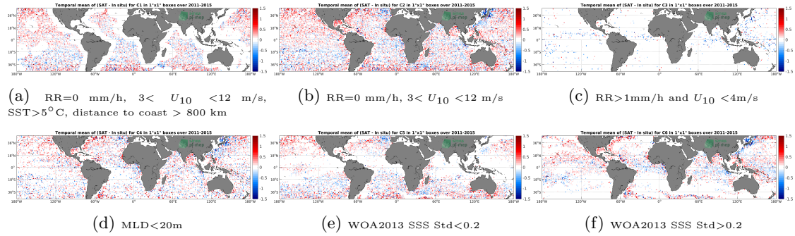
Figure 12: Temporal mean gridded over spatial boxes of size 1^\circ \times 1^\circ of \Delta SSS (Aquarius SSS L2 CAP v5 (JPL) - Argo) for 6 different subdatasets corresponding to: RR=0 mm/h, 3 < U_{10} < 12 m/s, SST > 5^\circ C , distance to coast > 800 km (a), RR=0 mm/h, 3 < U_{10} < 12 m/s (b), RR > 1 mm/h and U_{10} < 4 m/s (c), MLD < 20 m (d), WOA2013 SSS Std < 0.2 (e), WOA2013 SSS Std > 0.2 (f).
