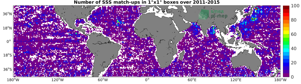
Figure 4: Number of SSS match-ups between Argo SSS and the Aquarius SSS L2 CAP v5 (JPL) SSS product for the Mid-Low Latitudes 45N-45S Pi-MEP region over 1°x1° boxes and for the full satellite product period.
