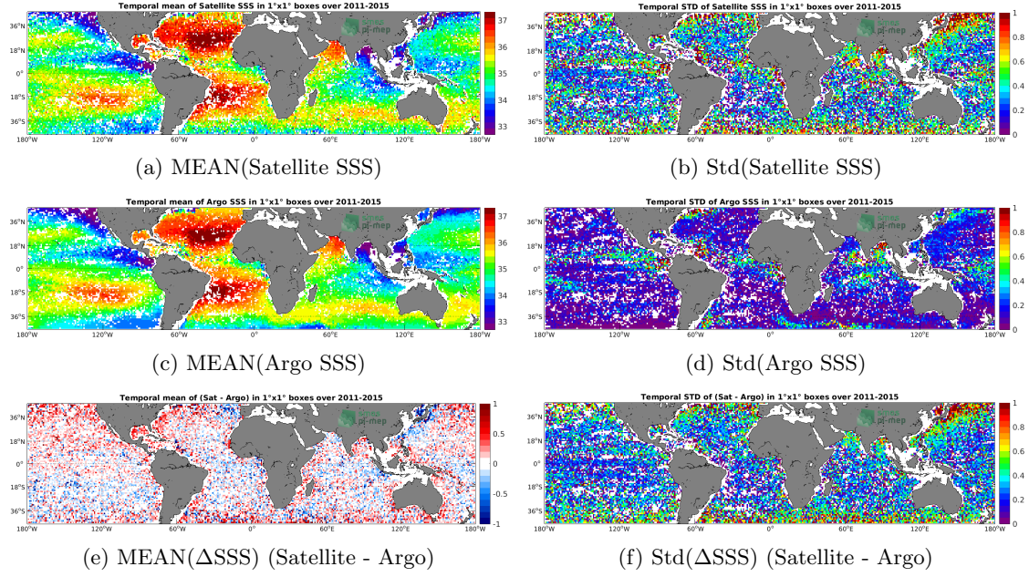
Figure 6: Temporal mean (left) and Std (right) of SSS from Aquarius SSS L2 CAP v5 (JPL) (top), Argo (middle), and of \Delta SSS (Satellite - Argo). Only match-up pairs are used to generate these maps.
