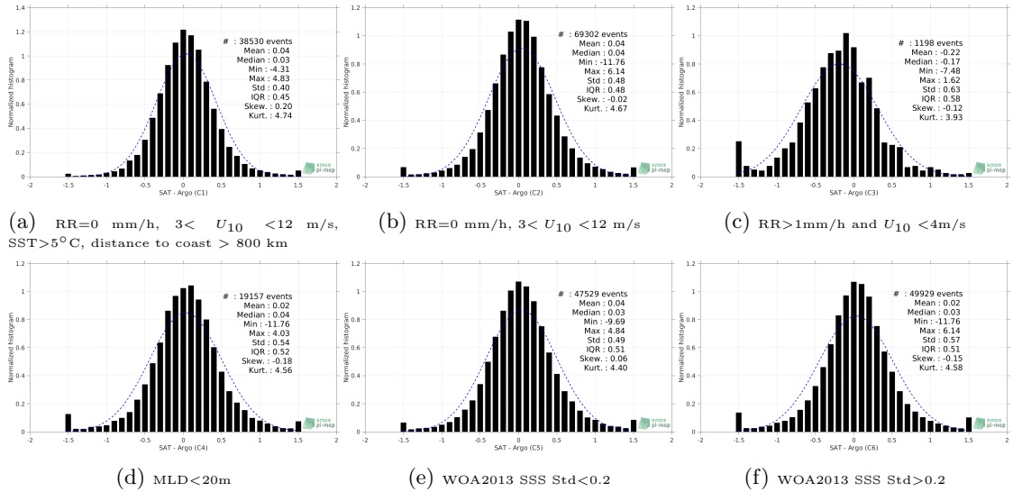
Figure 13: Normalized histogram of \Delta SSS (Aquarius-L2-JPL-V5 - Argo) for 6 different subdatasets corresponding to: RR=0 mm/h, 3 < U_{10} < 12 m/s, SST >5^\circ\text{C} , distance to coast > 800 km (a), RR=0 mm/h, 3 < U_{10} < 12 m/s (b), RR >1 mm/h and U_{10} < 4 m/s (c), MLD <20 m (d), WOA2013 SSS Std <0.2 (e), WOA2013 SSS Std >0.2 (f).
