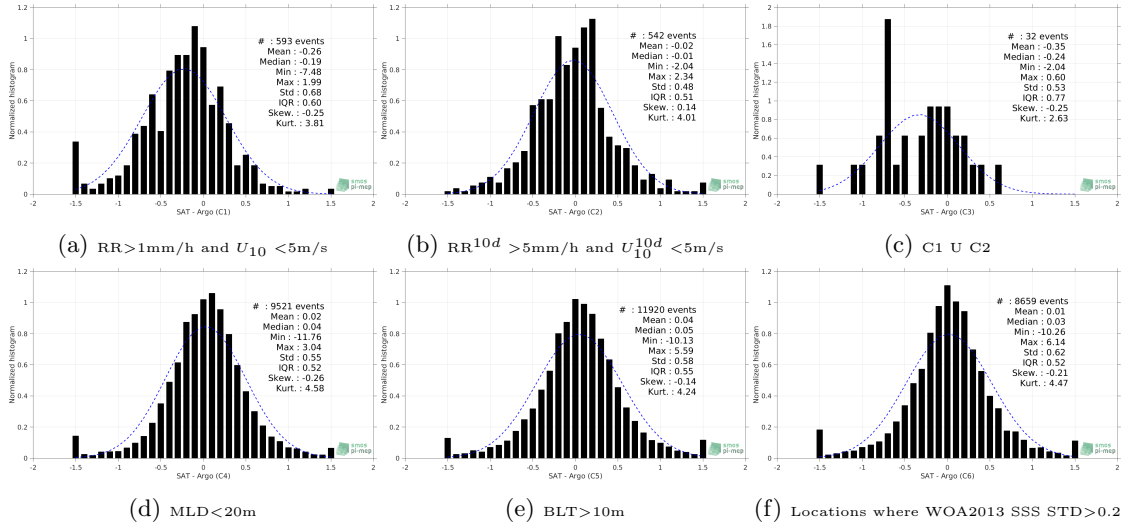
Figure 13: Normalized histogram of \Delta\text{SSS} (Aquarius-L2-JPL-V5 - Argo) for 6 different subdatasets corresponding to: \text{RR} > 1\text{mm/h} and U_{10} < 5\text{m/s} (a), \text{RR}^{10d} > 5\text{mm/h} and U_{10}^{10d} < 5\text{m/s} (b), C1 U C2 (c), \text{MLD} < 20\text{m} (d), \text{BLT} > 10\text{m} (e), Locations where WOA2013 SSS STD > 0.2 (f).
