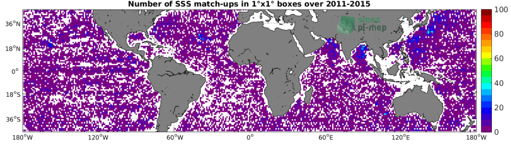
Figure 4: Number of SSS match-ups between Argo SSS and the Aquarius-L2-JPL-V5 SSS product for the Mid-Low Latitudes 45N-45S Pi-MEP region over 1°x1° boxes and for the full satellite product period.
