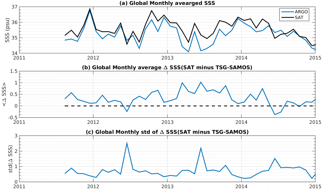
Figure 7: Time series of the monthly averaged mean SSS (top), mean \Delta SSS (Satellite - TSG-SAMOS) and STD of \Delta SSS (Satellite - TSG-SAMOS) over the Mid-Low Latitudes 45N-45S Pi-MEP region considering all match-ups collected by the Pi-MEP platform.
