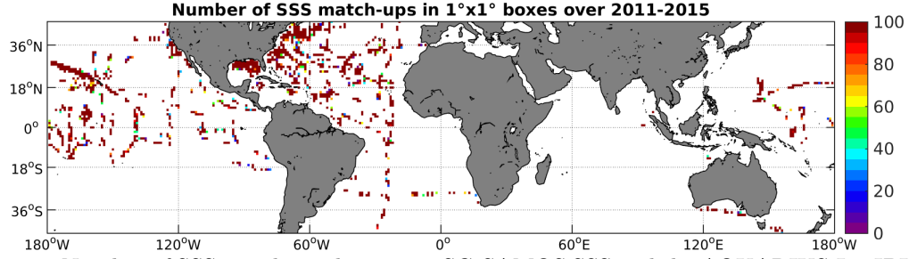
Figure 4: Number of SSS match-ups between TSG-SAMOS SSS and the AQUARIUS-L2-JPL-V4 SSS product for the Mid-Low Latitudes 45N-45S Pi-MEP region over 1^\circ \times 1^\circ boxes and for the full satellite product period.
