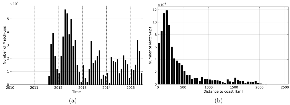
Figure 1: Number of match-ups between TSG-SAMOS and AQUARIUS-L2-JPL-V4 SSS as a function of time (a) and as function of the distance to coast (b) over the Mid-Low Latitudes 45N-45S Pi-MEP region and for the full satellite product period.
