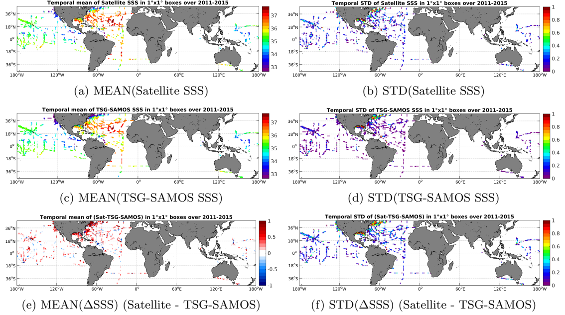
Figure 6: Temporal mean (left) and STD (right) of SSS from AQUARIUS-L2-JPL-V4 (top), TSG-SAMOS (middle), and of \Delta SSS (Satellite - TSG-SAMOS). Only match-up pairs are used to generate these maps.
