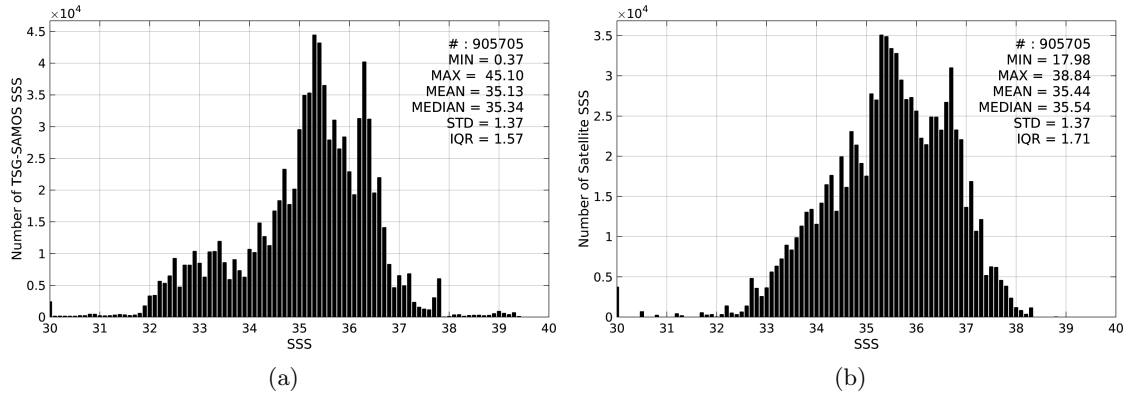
Figure 2: Histograms of SSS from TSG-SAMOS (a) and AQUARIUS-L2-JPL-V4 (b) considering all match-up pairs per bins of 0.1 over the Mid-Low Latitudes 45N-45S Pi-MEP region and for the full satellite product period.
