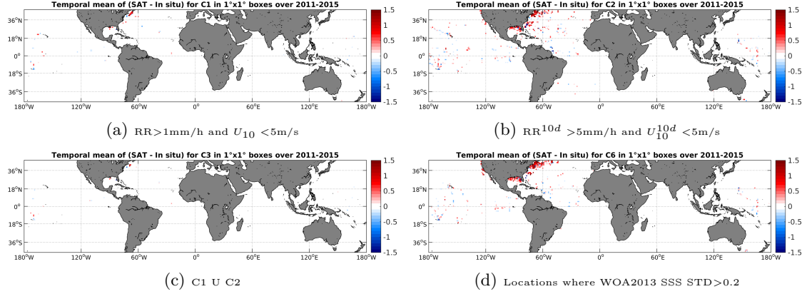
Figure 12: Temporal mean gridded over spatial boxes of size 1^\circ \times 1^\circ of \Delta SSS (AQUARIUS-L2-JPL-V4 - TSG-SAMOS) for 4 different subdatasets corresponding to: RR > 1\text{mm/h} and U_{10} < 5\text{m/s} (a), RR^{10d} > 5\text{mm/h} and U_{10}^{10d} < 5\text{m/s} (b), C1 U C2 (c), Locations where WOA2013 SSS STD > 0.2 (d).
