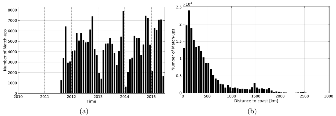
Figure 1: Number of match-ups between TSG-LEGOS-DM and AQUARIUS-L2-JPL-V4 SSS as a function of time (a) and as function of the distance to coast (b) over the Mid-Low Latitudes 45N-45S Pi-MEP region and for the full satellite product period.
