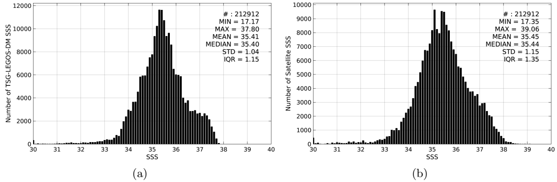
Figure 2: Histograms of SSS from TSG-LEGOS-DM (a) and AQUARIUS-L2-JPL-V4 (b) considering all match-up pairs per bins of 0.1 over the Mid-Low Latitudes 45N-45S Pi-MEP region and for the full satellite product period.
