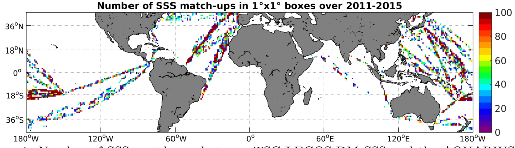
Figure 4: Number of SSS match-ups between TSG-LEGOS-DM SSS and the AQUARIUS-L2-JPL-V4 SSS product for the Mid-Low Latitudes 45N-45S Pi-MEP region over 1°x1° boxes and for the full satellite product period.
