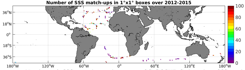
Figure 4: Number of SSS match-ups between TSG-GOSUD-Sailing-ship SSS and the AQUARIUS-L2-JPL-V4 SSS product for the Mid-Low Latitudes 45N-45S Pi-MEP region over 1^\circ \times 1^\circ boxes and for the full satellite product period.
