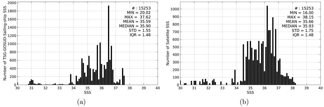
Figure 2: Histograms of SSS from TSG-GOSUD-Sailing-ship (a) and AQUARIUS-L2-JPL-V4 (b) considering all match-up pairs per bins of 0.1 over the Mid-Low Latitudes 45N-45S Pi-MEP region and for the full satellite product period.
