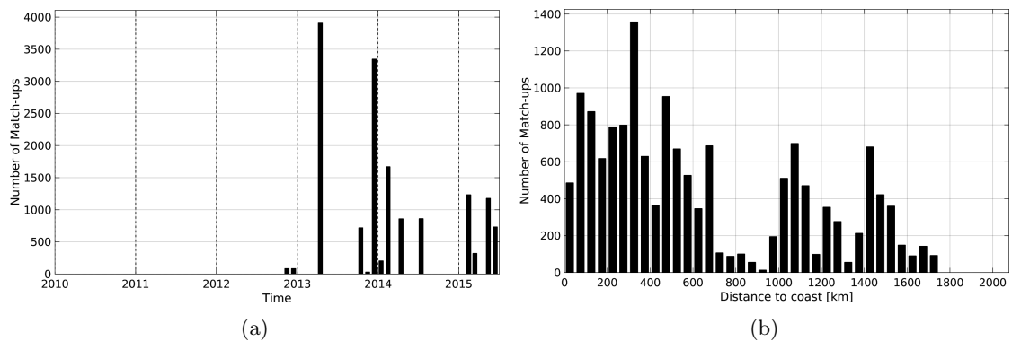
Figure 1: Number of match-ups between TSG-GOSUD-Sailing-ship and AQUARIUS-L2-JPL-V4 SSS as a function of time (a) and as function of the distance to coast (b) over the Mid-Low Latitudes 45N-45S Pi-MEP region and for the full satellite product period.
