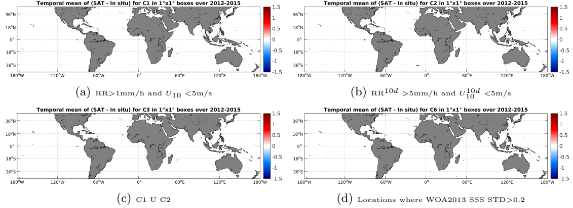
Figure 12: Temporal mean gridded over spatial boxes of size 1^\circ \times 1^\circ of \Delta SSS (AQUARIUS-L2-JPL-V4 - TSG-GOSUD-Sailing-ship) for 4 different subdatasets corresponding to: RR > 1 mm/h and U_{10} < 5 m/s (a), RR^{10d} > 5 mm/h and U_{10}^{10d} < 5 m/s (b), C1 U C2 (c), Locations where WOA2013 SSS STD > 0.2 (d).
