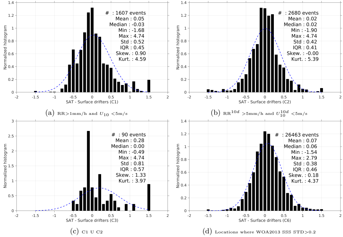
Figure 12: Normalized histogram of \Delta\text{SSS} (AQUARIUS-L2-JPL-V4 - Surface drifters) for 6 different subdatasets corresponding to: \text{RR} > 1\text{mm/h} and U_{10} < 5\text{m/s} (a), \text{RR}^{10d} > 5\text{mm/h} and U_{10}^{10d} < 5\text{m/s} (b), C1 U C2 (c), Locations where WOA2013 SSS STD > 0.2 (d).
