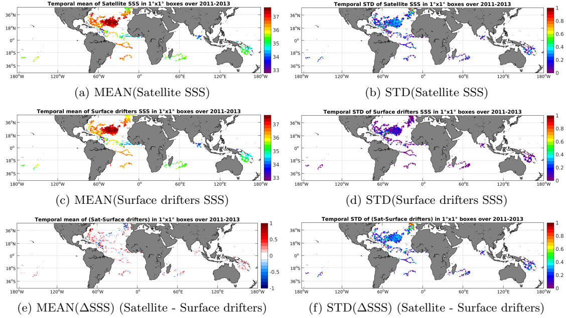
Figure 5: Temporal mean (left) and STD (right) of SSS from AQUARIUS-L2-JPL-V4 (top), Surface drifters (middle), and of \Delta SSS (Satellite - Surface drifters). Only match-up pairs are used to generate these maps.
