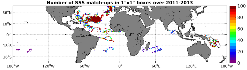
Figure 3: Number of SSS match-ups between Surface drifters SSS and the AQUARIUS-L2-JPL-V4 SSS product for the Mid-Low Latitudes 45N-45S Pi-MEP region over 1^\circ \times 1^\circ boxes and for the full satellite product period.
