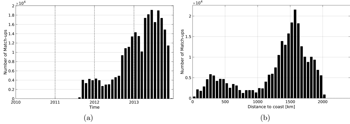
Figure 1: Number of match-ups between Surface drifters and AQUARIUS-L2-JPL-V4 SSS as a function of time (a) and as function of the distance to coast (b) over the Mid-Low Latitudes 45N-45S Pi-MEP region and for the full satellite product period.
