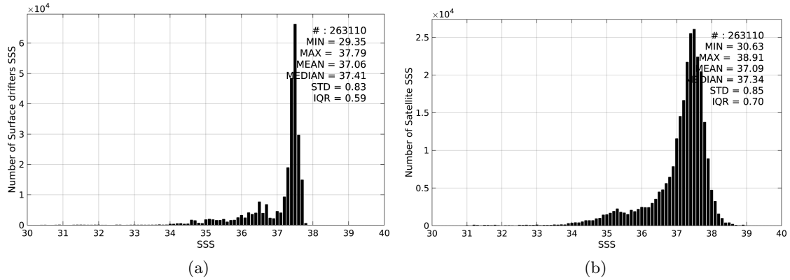
Figure 2: Histograms of SSS from Surface drifters (a) and AQUARIUS-L2-JPL-V4 (b) considering all match-up pairs per bins of 0.1 over the Mid-Low Latitudes 45N-45S Pi-MEP region and for the full satellite product period.
