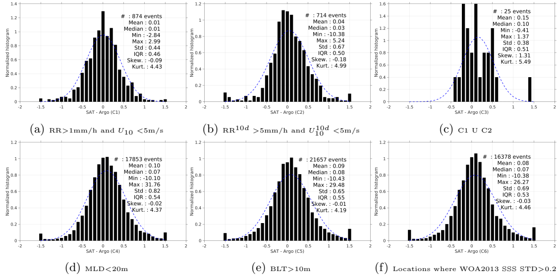
Figure 13: Normalized histogram of \Delta\text{SSS} (AQUARIUS-L2-JPL-V4 - Argo) for 6 different subdatasets corresponding to: \text{RR} > 1\text{mm/h} and U_{10} < 5\text{m/s} (a), \text{RR}^{10d} > 5\text{mm/h} and U_{10}^{10d} < 5\text{m/s} (b), C1 U C2 (c), \text{MLD} < 20\text{m} (d), \text{BLT} > 10\text{m} (e), Locations where WOA2013 SSS STD > 0.2 (f).
