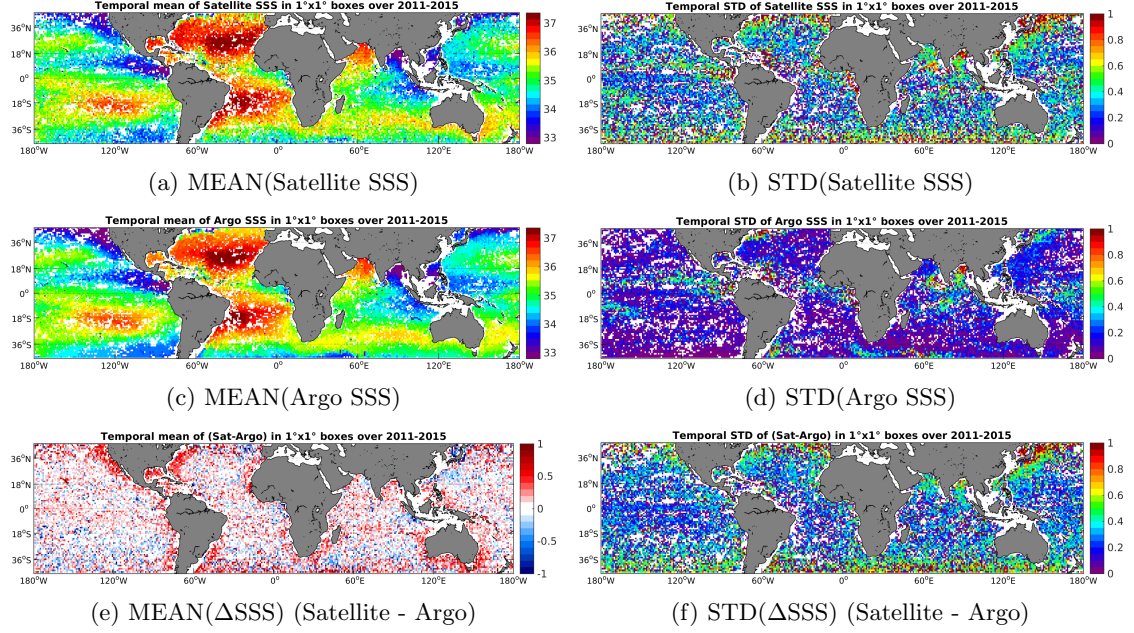
Figure 6: Temporal mean (left) and STD (right) of SSS from AQUARIUS-L2-JPL-V4 (top), Argo (middle), and of \Delta SSS (Satellite - Argo). Only match-up pairs are used to generate these maps.
