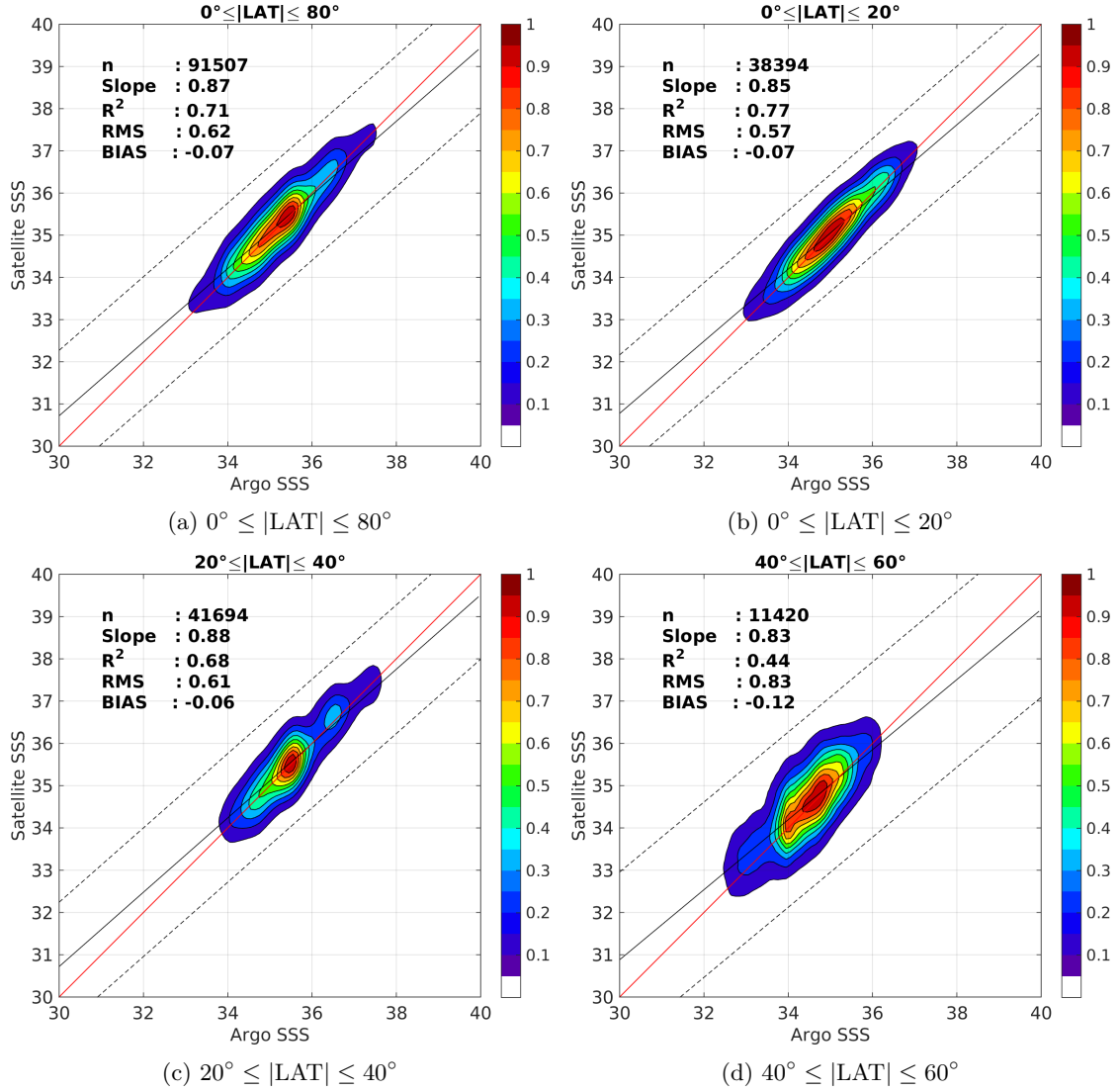
Figure 9: Contour maps of the concentration of AQUARIUS-L2-JPL-V4 SSS (y-axis) versus Argo SSS (x-axis) at match-up pairs for different latitude bands. For each plot, the red line shows x=y . The black thin and dashed lines indicate a linear fit through the data cloud and the \pm 95\% confidence levels, respectively. The number match-up pairs n , the slope and R^2 coefficient of the linear fit, the root mean square (RMS) and the mean bias between satellite and in situ data are indicated for each latitude band in each plots.
