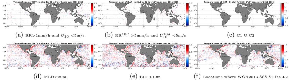
Figure 12: Temporal mean gridded over spatial boxes of size 1^\circ \times 1^\circ of \Delta\text{SSS} (AQUARIUS-L2-JPL-V4 - Argo) for 6 different subdatasets corresponding to: \text{RR} > 1\text{mm/h} and U_{10} < 5\text{m/s} (a), \text{RR}^{10d} > 5\text{mm/h} and U_{10}^{10d} < 5\text{m/s} (b), C1 U C2 (c), \text{MLD} < 20\text{m} (d), \text{BLT} > 10\text{m} (e), Locations where WOA2013 SSS STD > 0.2 (f).
