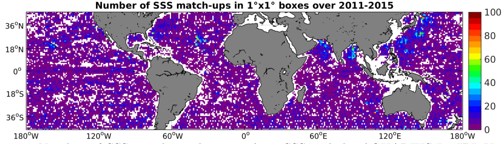
Figure 4: Number of SSS match-ups between Argo SSS and the AQUARIUS-L2-JPL-V4 SSS product for the Mid-Low Latitudes 45N-45S Pi-MEP region over 1^\circ \times 1^\circ boxes and for the full satellite product period.
