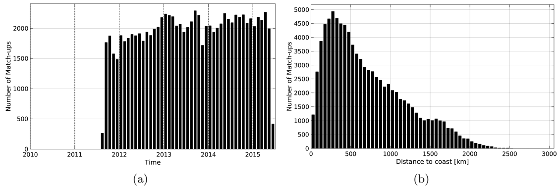
Figure 1: Number of match-ups between Argo and AQUARIUS-L2-JPL-V4 SSS as a function of time (a) and as function of the distance to coast (b) over the Mid-Low Latitudes 45N-45S Pi-MEP region and for the full satellite product period.
