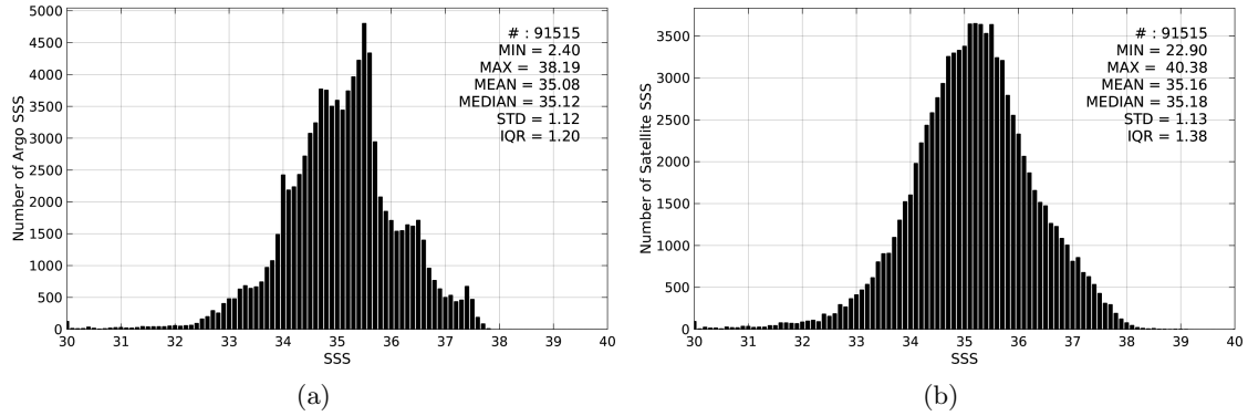
Figure 2: Histograms of SSS from Argo (a) and AQUARIUS-L2-JPL-V4 (b) considering all match-up pairs per bins of 0.1 over the Mid-Low Latitudes 45N-45S Pi-MEP region and for the full satellite product period.
