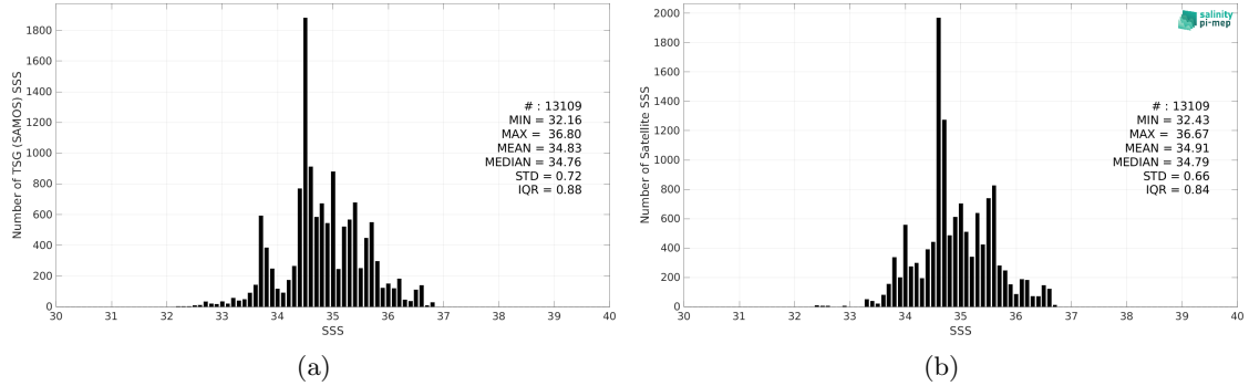
Figure 2: Histograms of SSS from TSG (SAMOS) (a) and SMOS and SMAP SSS L4 OI v1 - 7 Days (LOPS) (b) considering all match-up pairs per bins of 0.1 over the Indian Ocean Pi-MEP region and for the full satellite product period.
