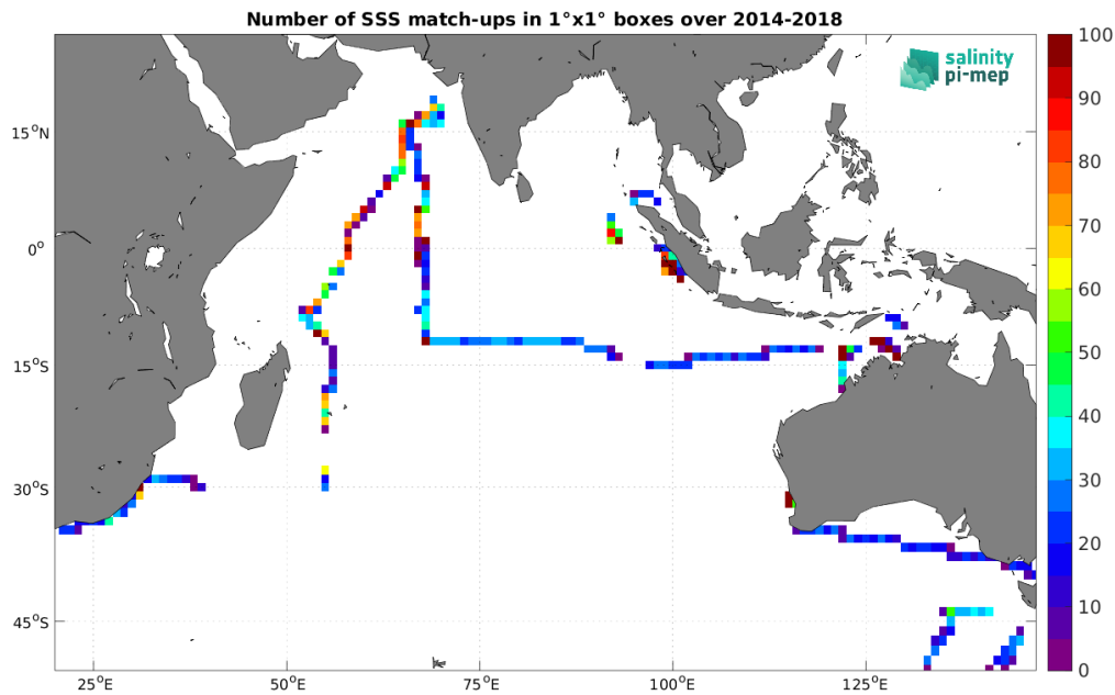
Figure 4: Number of SSS match-ups between TSG (SAMOS) SSS and the SMOS and SMAP SSS L4 OI v1 - 7 Days (LOPS) SSS product for the Indian Ocean Pi-MEP region over 1^\circ \times 1^\circ boxes and for the full satellite product period.
