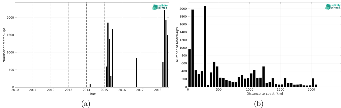
Figure 1: Number of match-ups between TSG (SAMOS) and SMOS and SMAP SSS L4 OI v1 - 7 Days (LOPS) SSS as a function of time (a) and as function of the distance to coast (b) over the Indian Ocean Pi-MEP region and for the full satellite product period.
