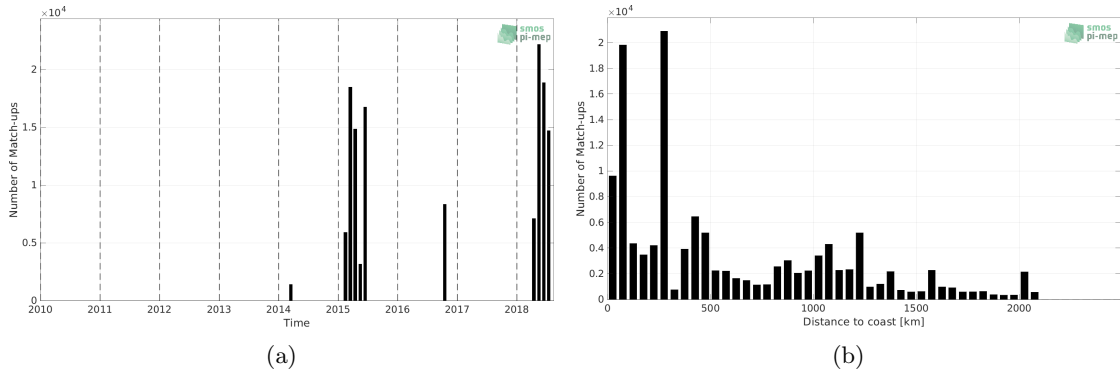
Figure 1: Number of match-ups between TSG (SAMOS) and SMOS and SMAP SSS L4 OI v1 - 7 Days (LOPS) SSS as a function of time (a) and as function of the distance to coast (b) over the Indian Ocean Pi-MEP region and for the full satellite product period.
