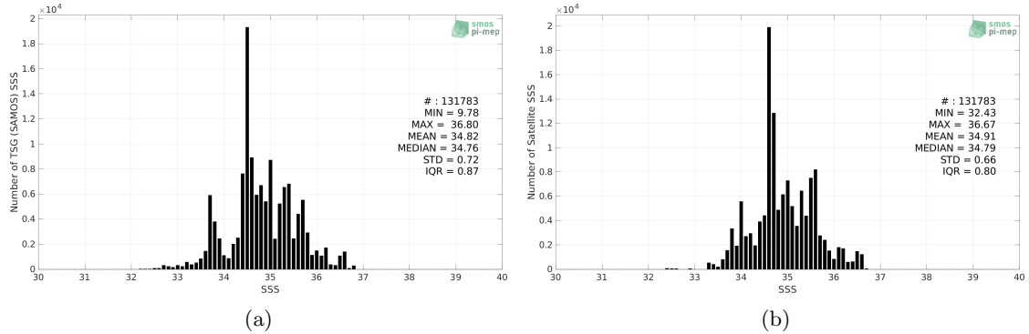
Figure 2: Histograms of SSS from TSG (SAMOS) (a) and SMOS and SMAP SSS L4 OI v1 - 7 Days (LOPS) (b) considering all match-up pairs per bins of 0.1 over the Indian Ocean Pi-MEP region and for the full satellite product period.
