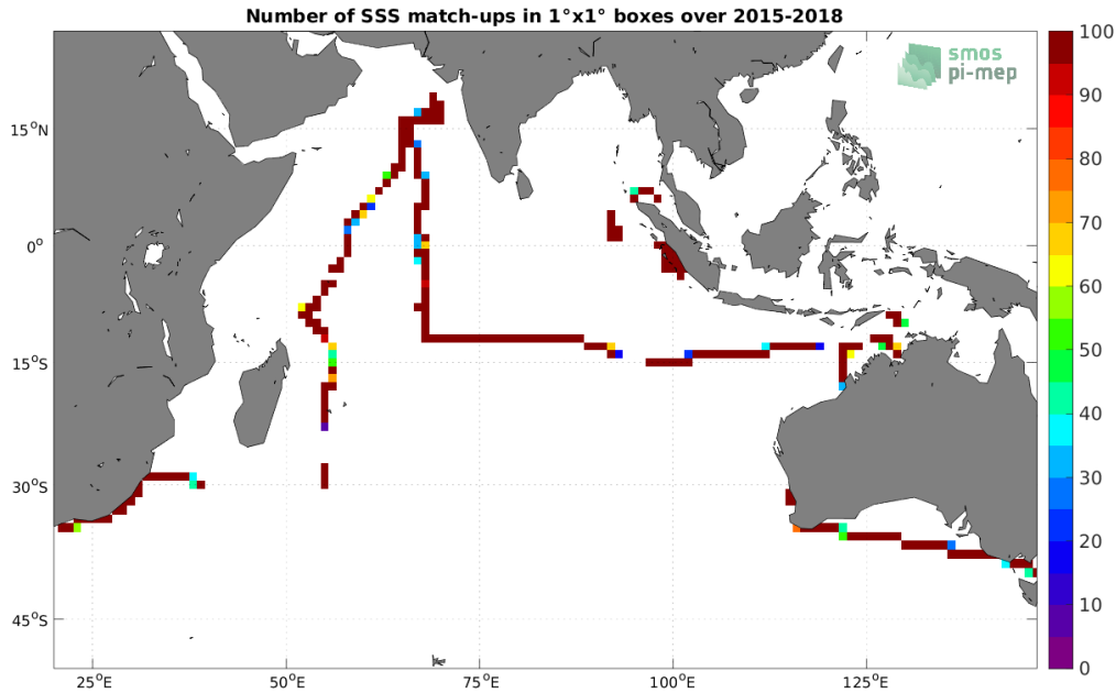
Figure 4: Number of SSS match-ups between TSG (SAMOS) SSS and the SMOS and SMAP SSS L4 OI v1 - 7 Days (LOPS) SSS product for the Indian Ocean Pi-MEP region over 1°x1° boxes and for the full satellite product period.
