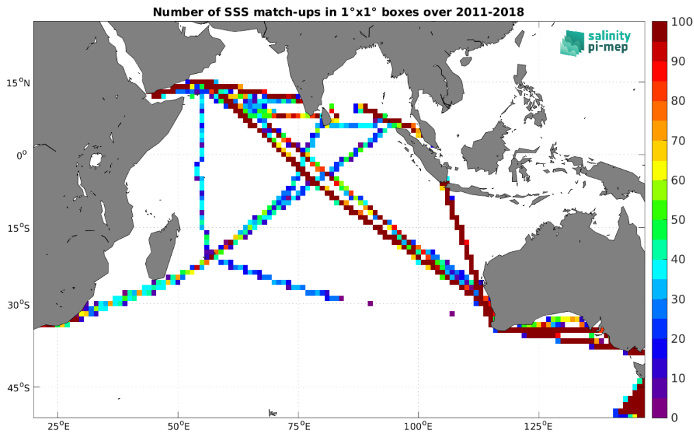
Figure 4: Number of SSS match-ups between TSG (LEGOS-DM) SSS and the SMOS and SMAP SSS L4 OI v1 - 7 Days (LOPS) SSS product for the Indian Ocean Pi-MEP region over 1^\circ \times 1^\circ boxes and for the full satellite product period.
